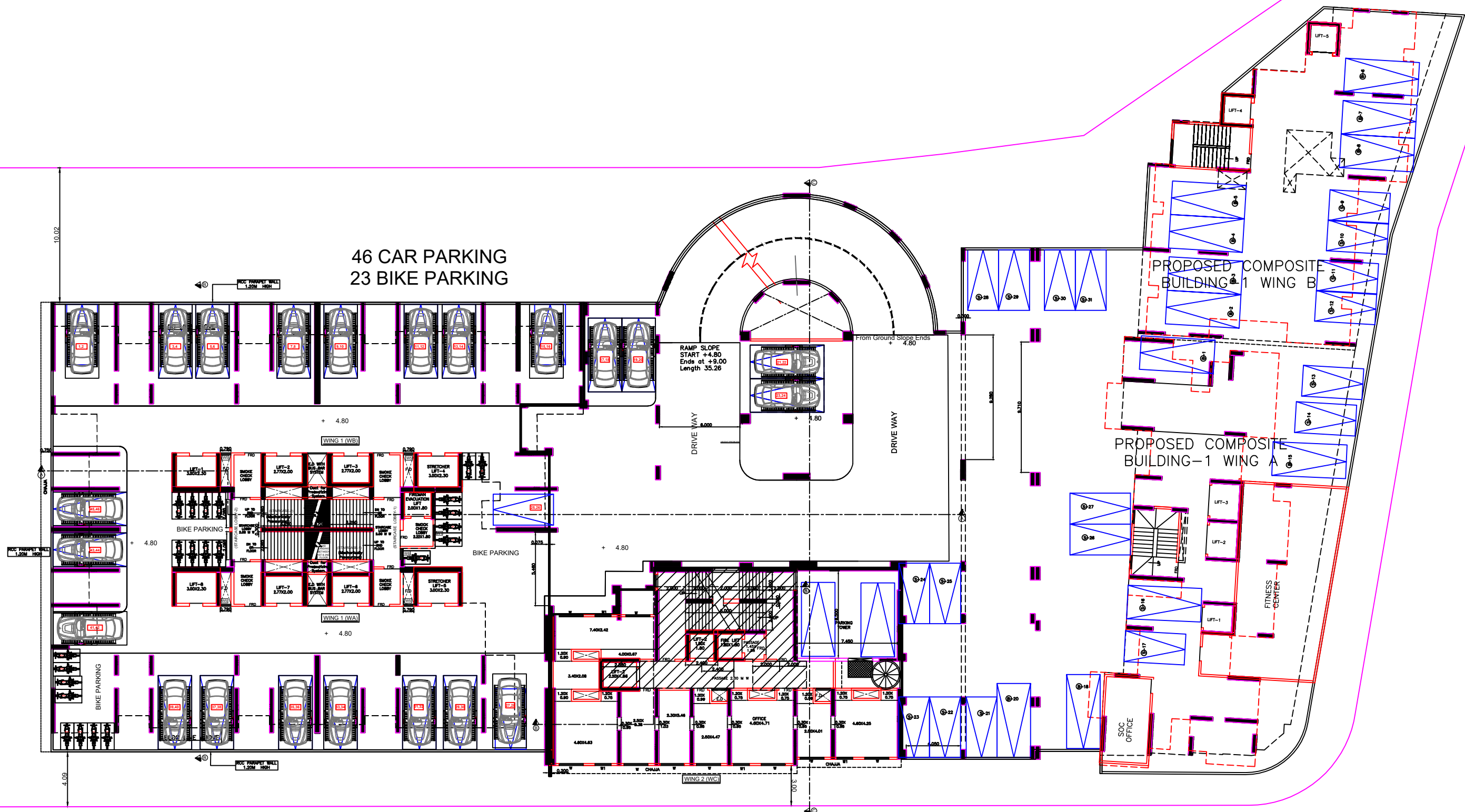
1ST PODIUM FLOOR PLAN WING 1 (WA&WB) & WING 2 (WC) SCALE 1:100
