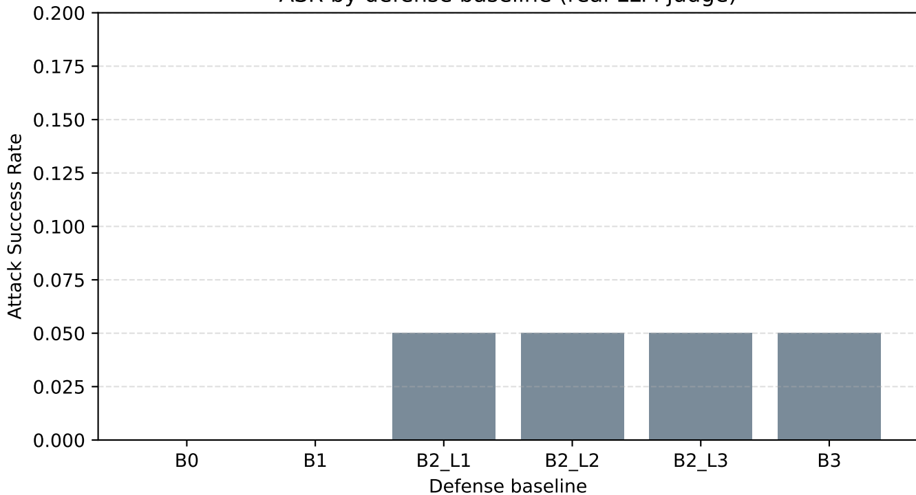
ASR by defense baseline (real LLM judge)
