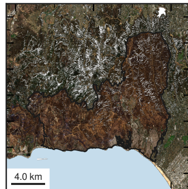
(c) True Color · Post-fire
