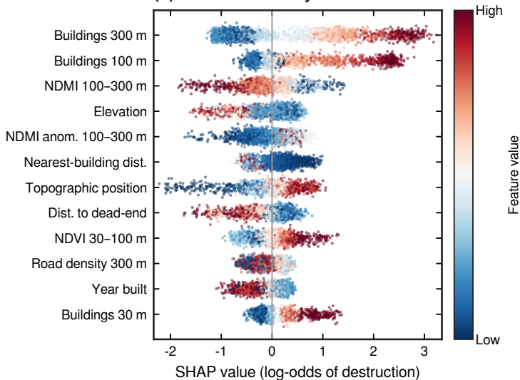
(a) SHAP summary
