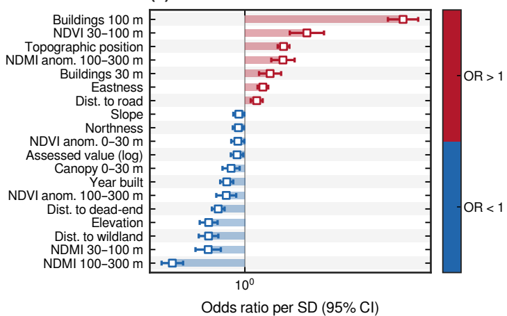
(c) Odds ratios
