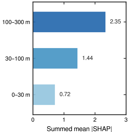
(b) SHAP by ring
