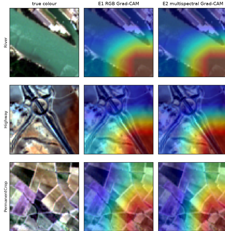
Figure 7: Grad-CAM for the RGB (E1) and multispectral (E2) models on three test patches. Both attend to the same discriminative regions, consistent with their near-identical full-data accuracy.
