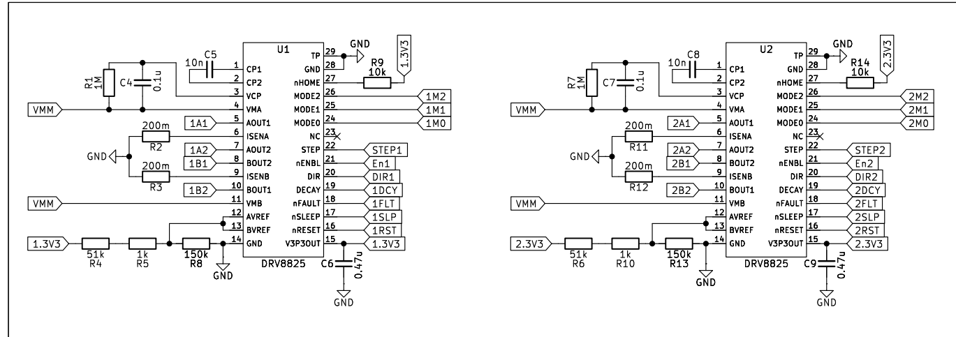
2xDRV8825 Step Motor Driver
