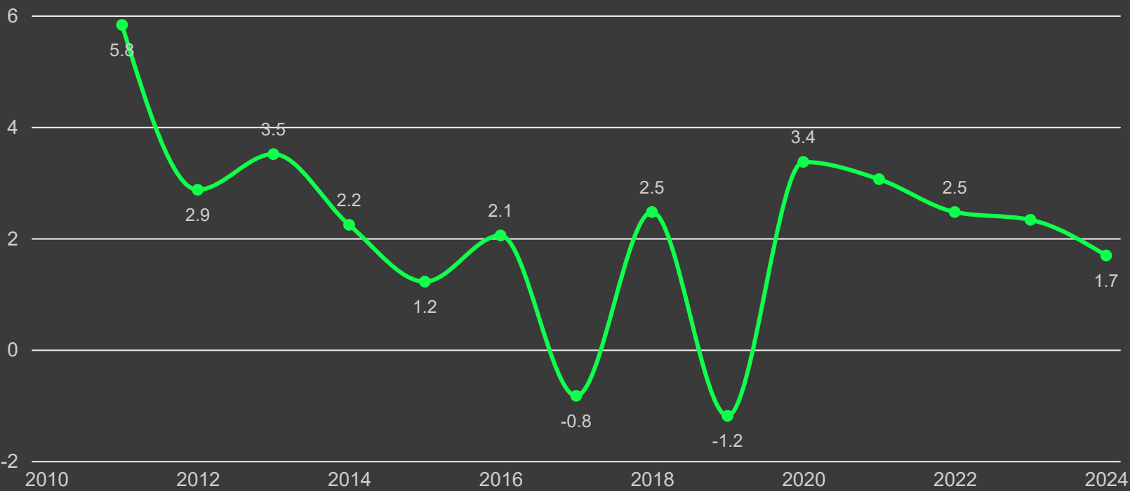
Inflation (%) over time
