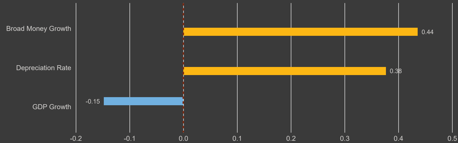
Coefficient Plot with 95% CI
