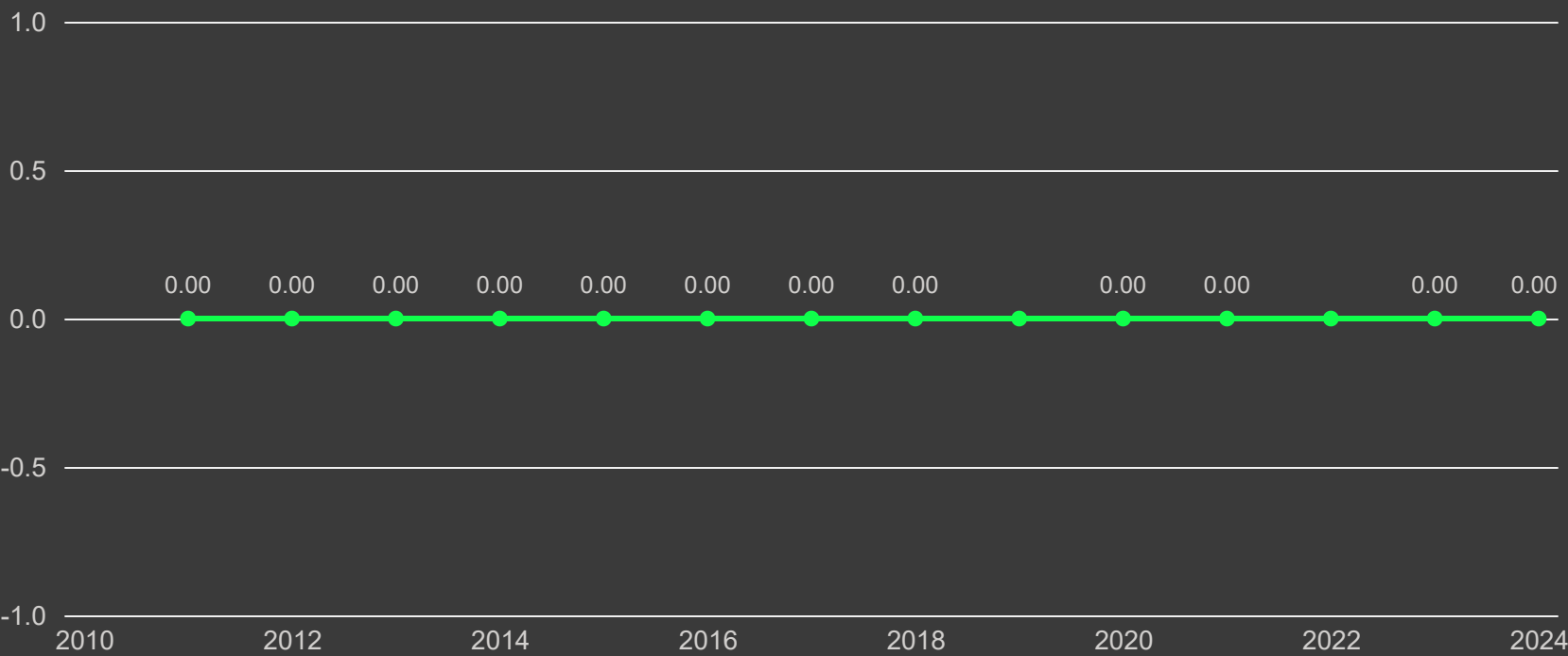
Depreciation Rate (%) over time
