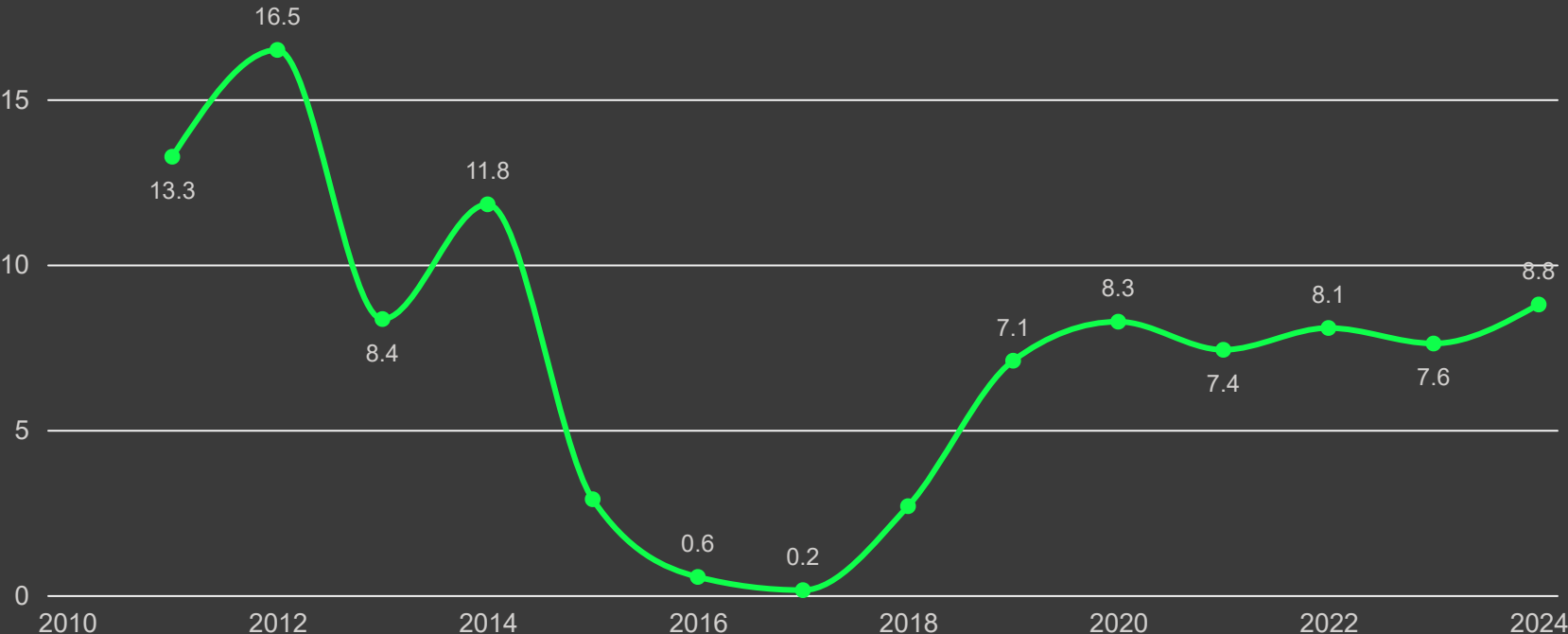
Broad Money Growth (%) over time
