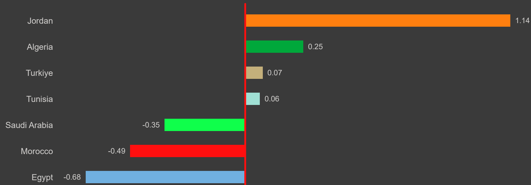
Country Fixed Effects ( \alpha_i )
