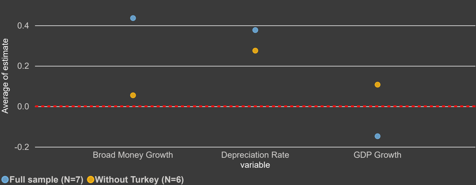
Sensitivity
