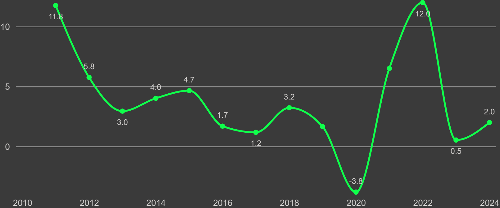
GDP Growth (%) over time
