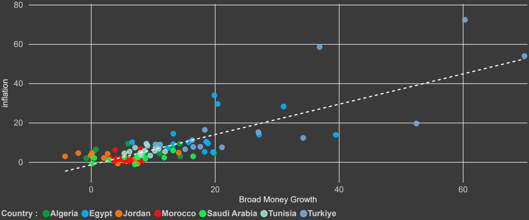
Broad Money vs Inflation
