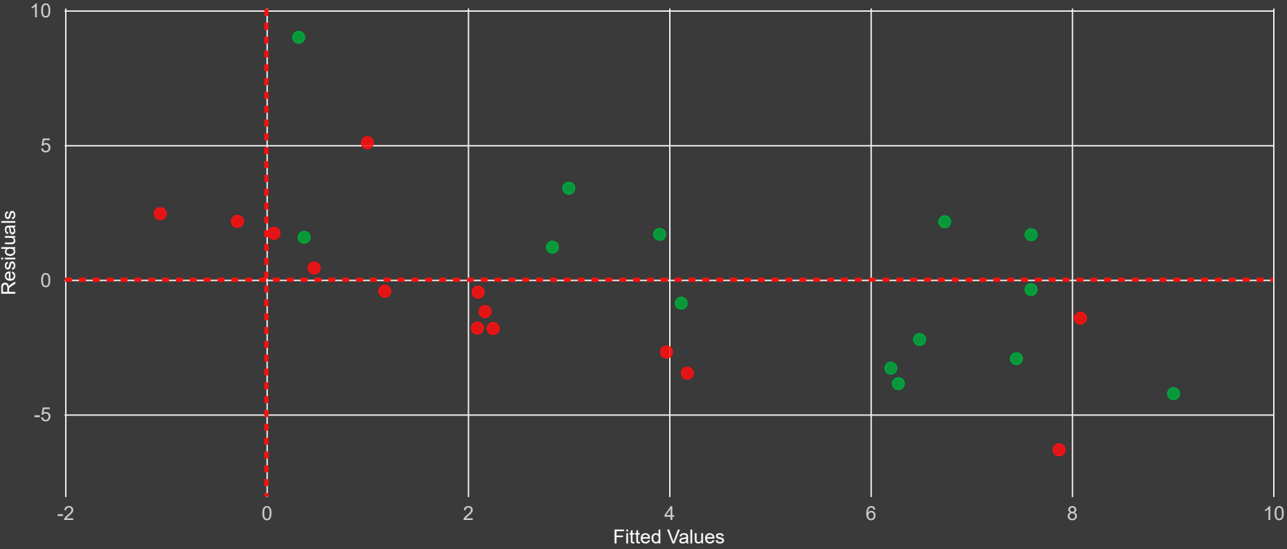
Residuals vs Fitted values
