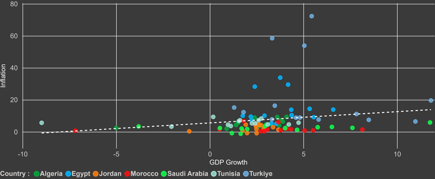
GDP Growth vs Inflation
