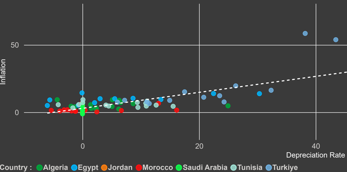
Depreciation Rate vs Inflation
