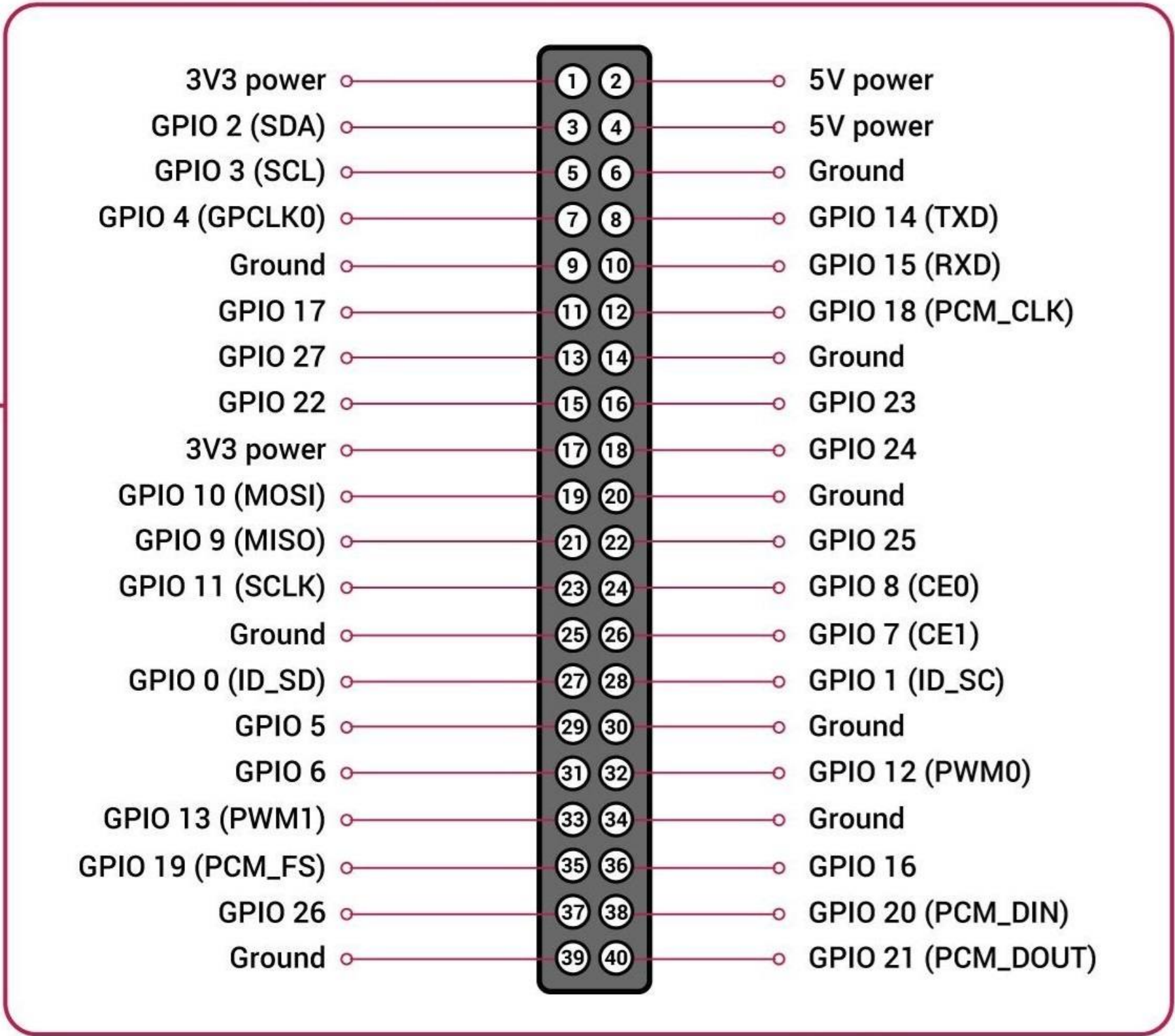
40 GPIO Pins Description of Raspberry Pi 5
