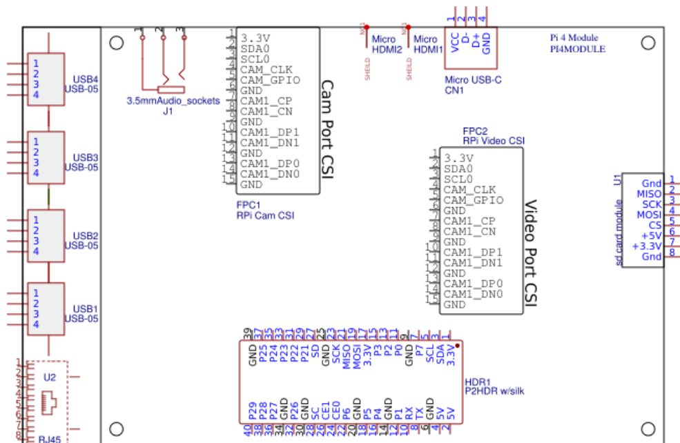
FIG 2.2 CIRCUIT DIAGRAM OF RASPBERRY PI 4(MODEL B)
