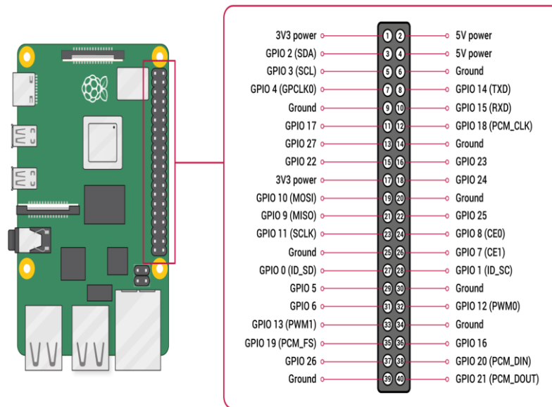
FIG 2.3 RASPBERRY PI 4 PINS
