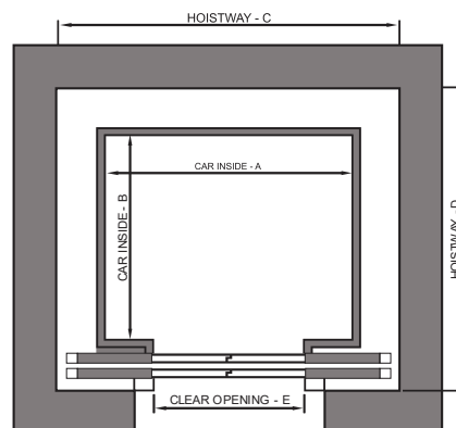
HOISTWAY PLAN
