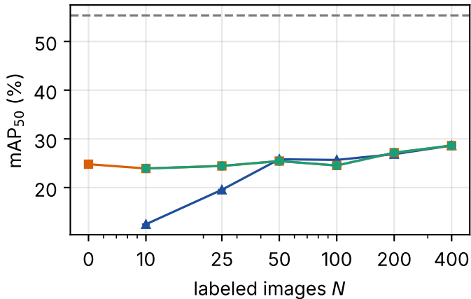
HomeObjects-3K
