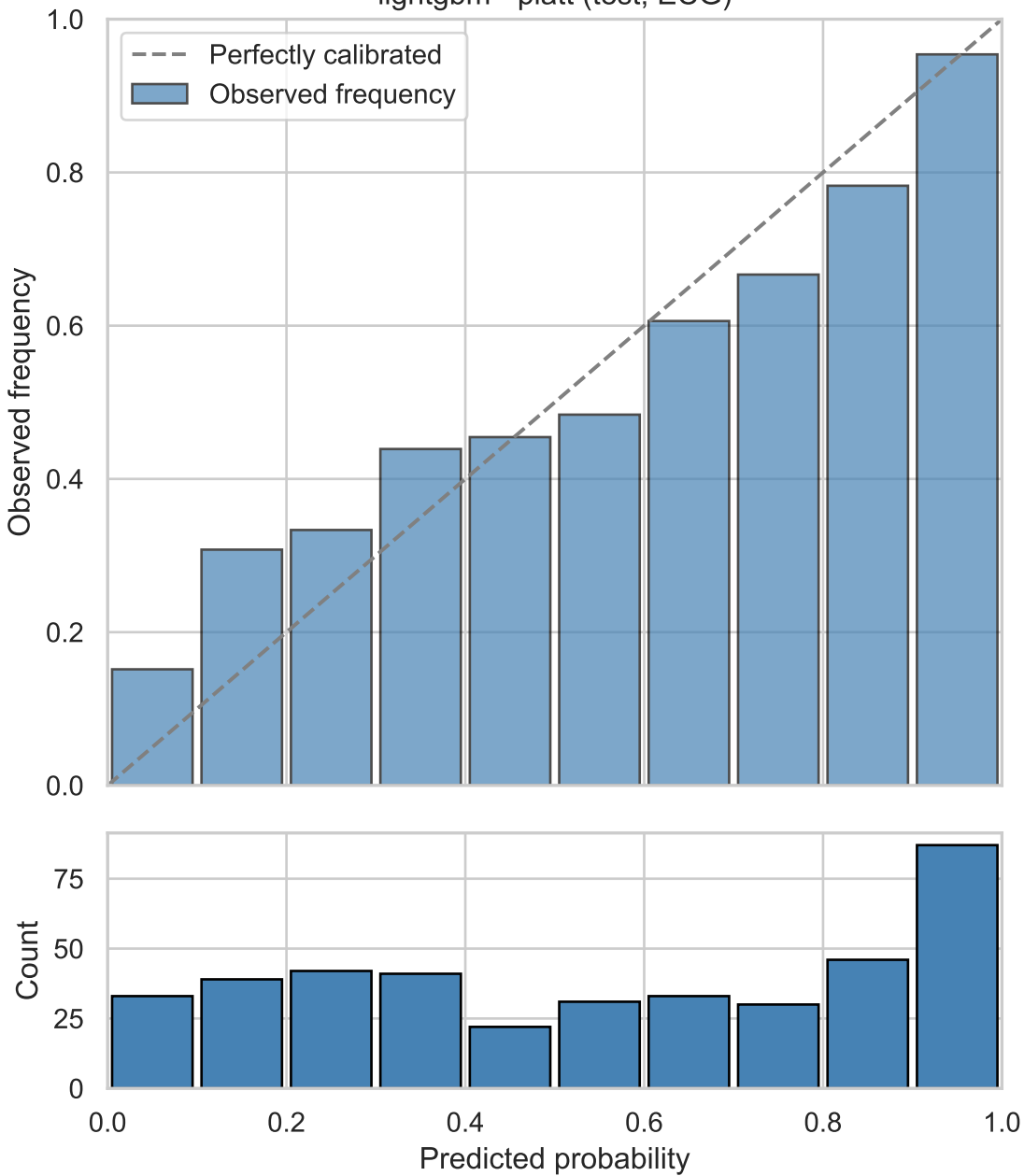
lightgbm - platt (test, ECG)
