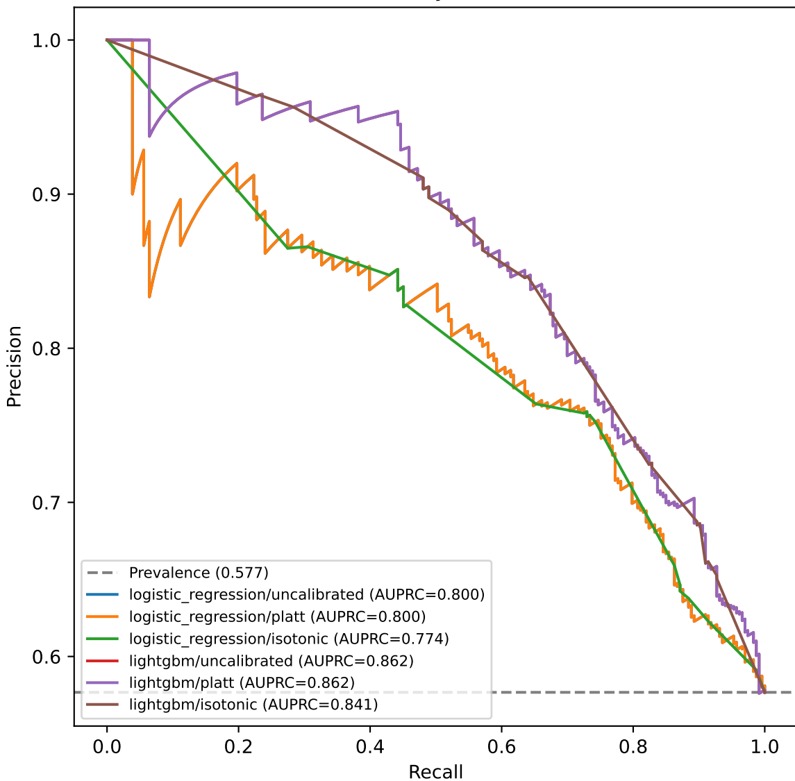
PR - ECG Abnormality Detection, Test Set
