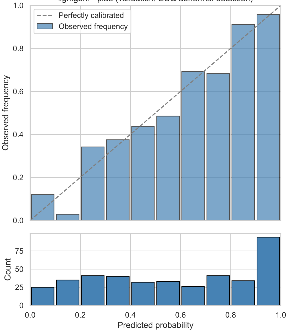
lightgbm - platt (validation, ECG abnormal detection)
