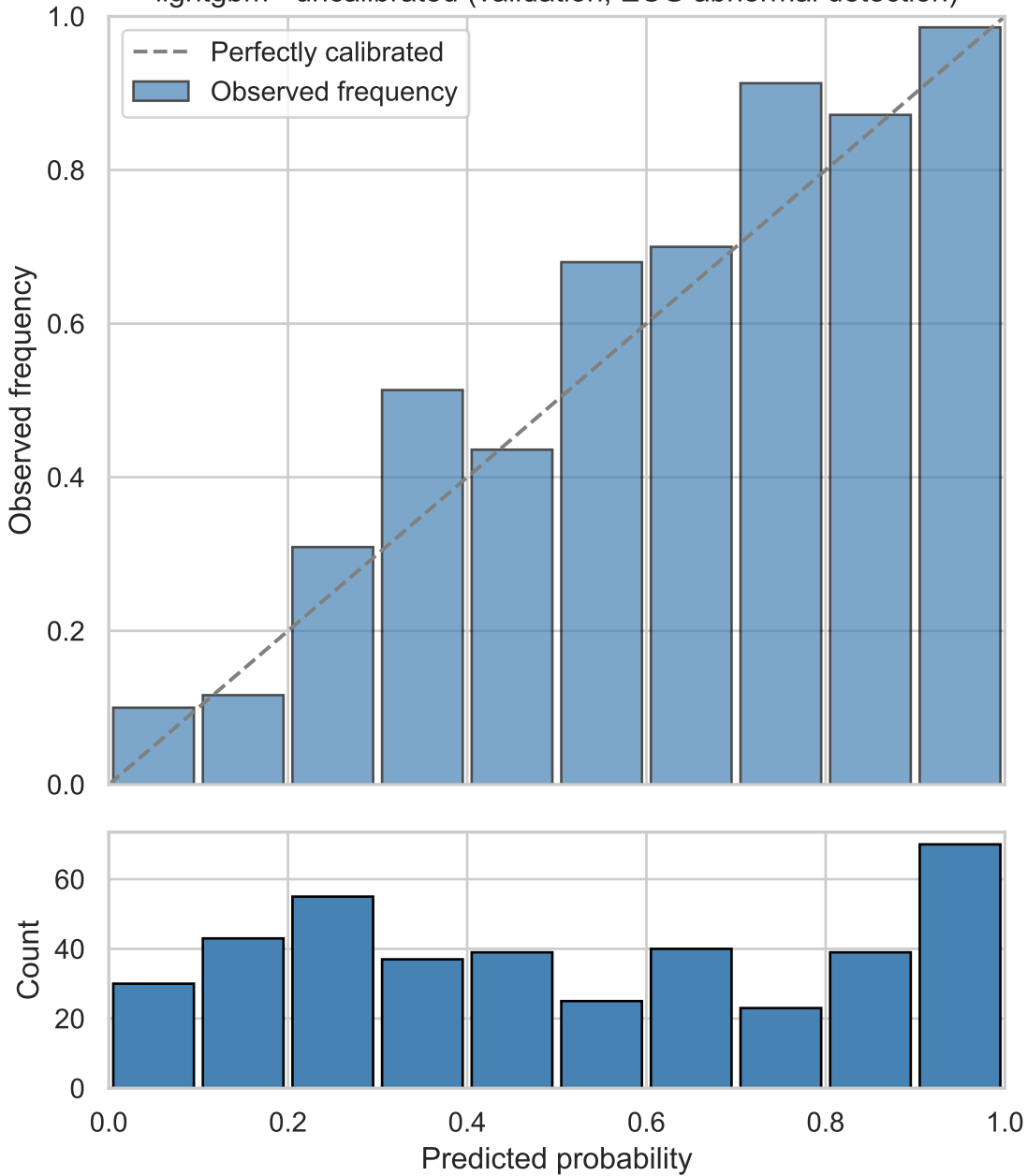
lightgbm - uncalibrated (validation, ECG abnormal detection)
