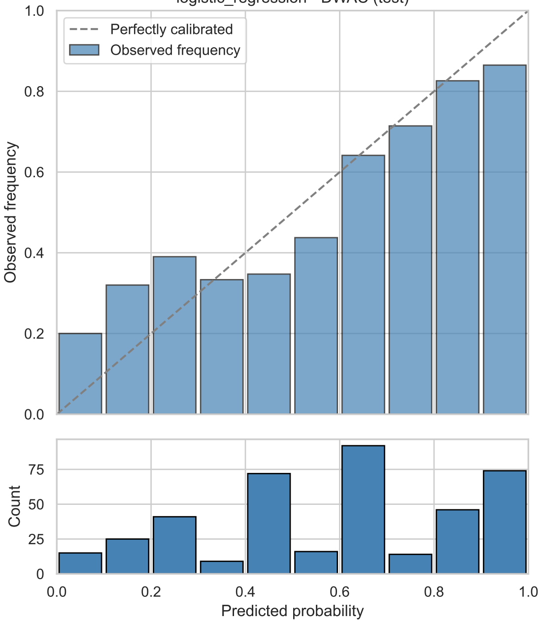
logistic_regression - DWAC (test)
