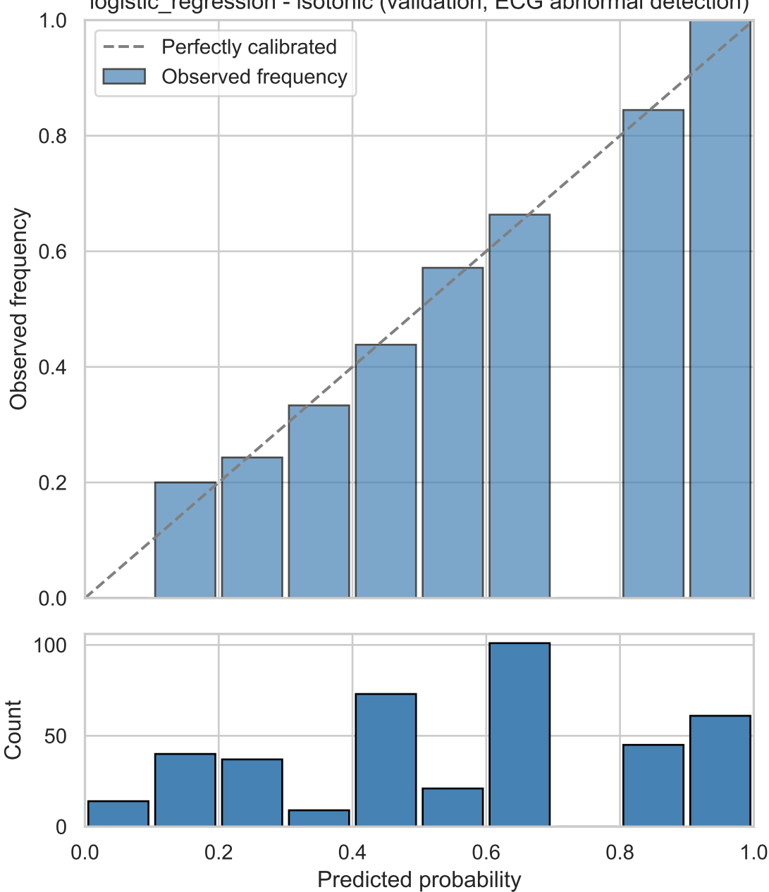
logistic_regression - isotonic (validation, ECG abnormal detection)
