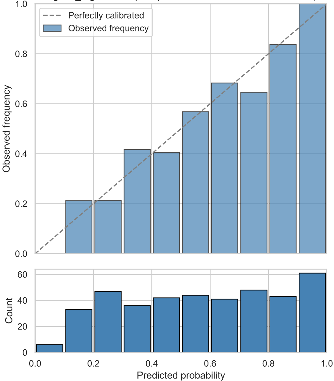
logistic_regression - platt (validation, ECG abnormal detection)
