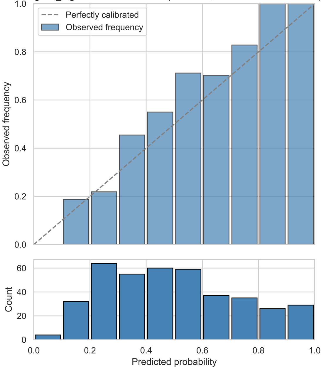
logistic_regression - uncalibrated (validation, ECG abnormal detection)
