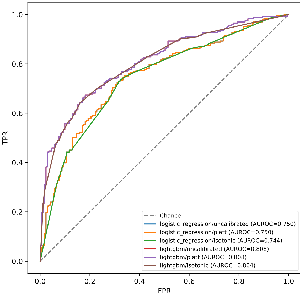
ROC - ECG Abnormality Detection, Test Set
