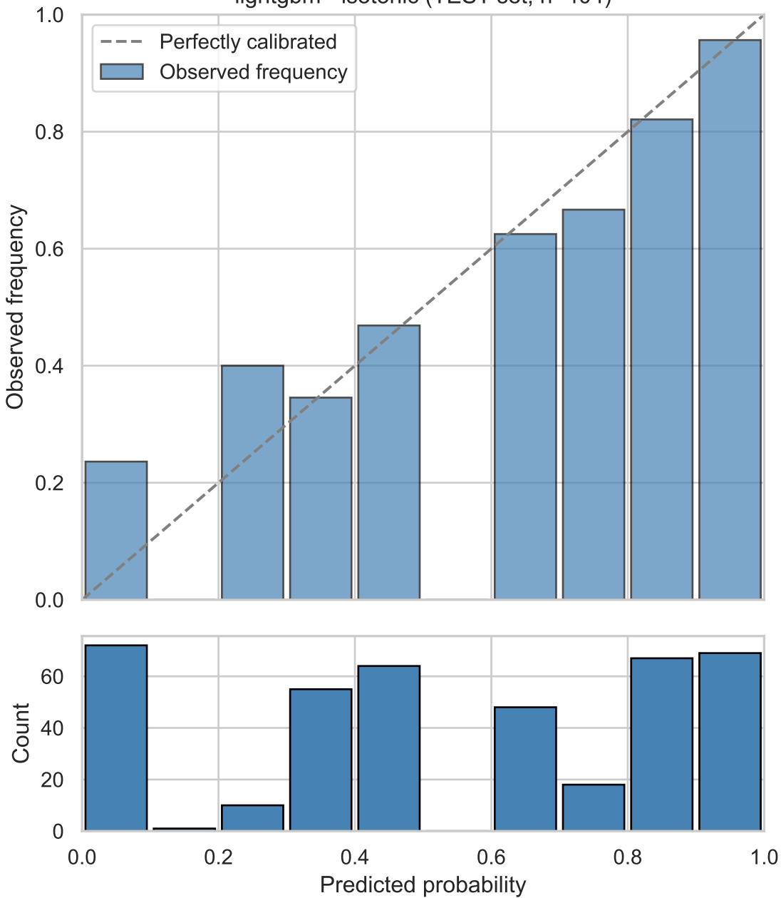
lightgbm - isotonic (TEST set, n=404)
