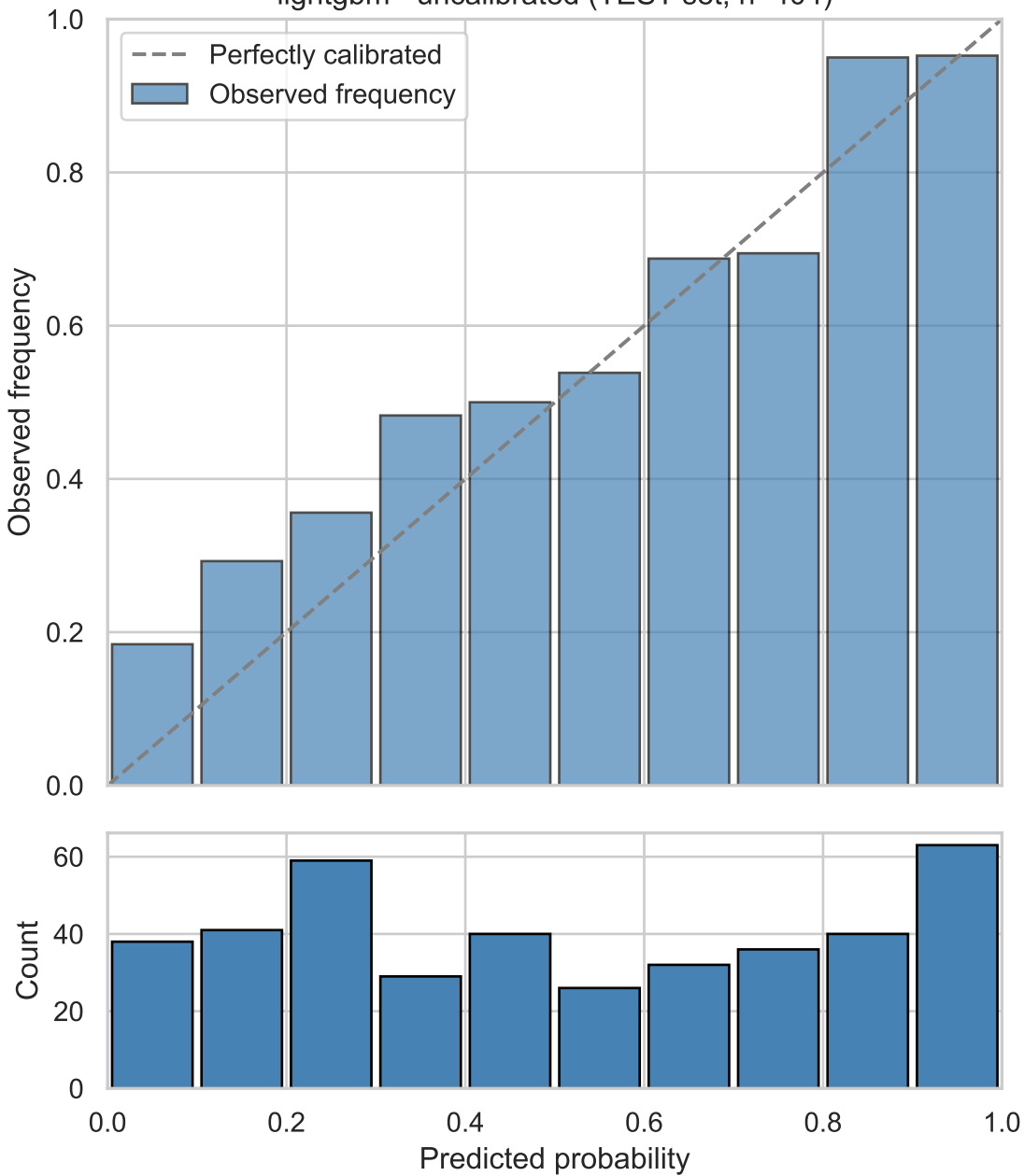
lightgbm - uncalibrated (TEST set, n=404)
