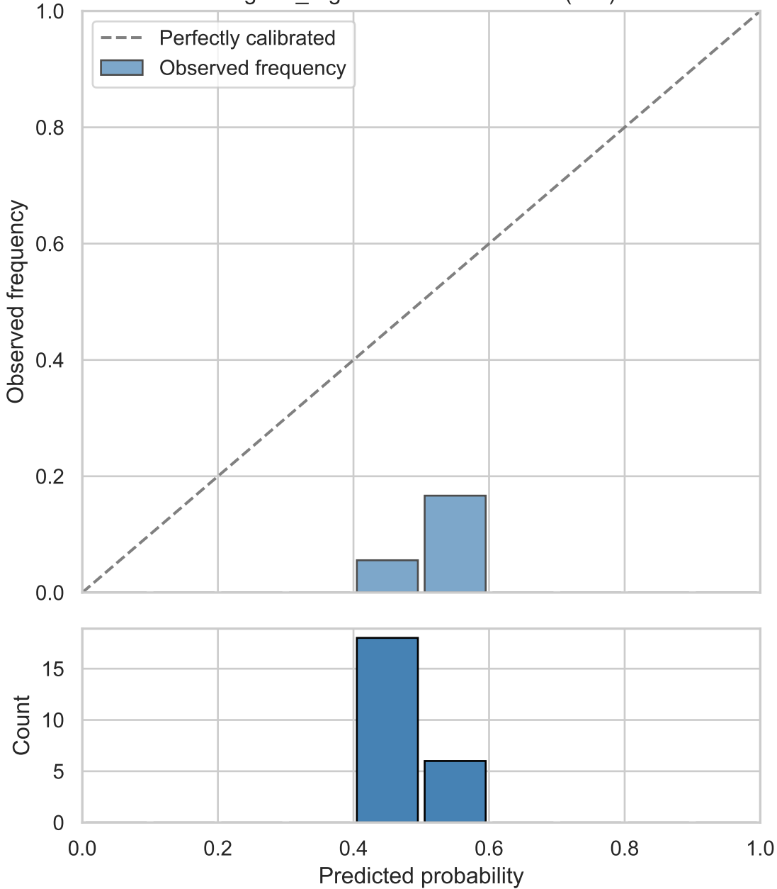
logistic_regression - uncalibrated (test)
