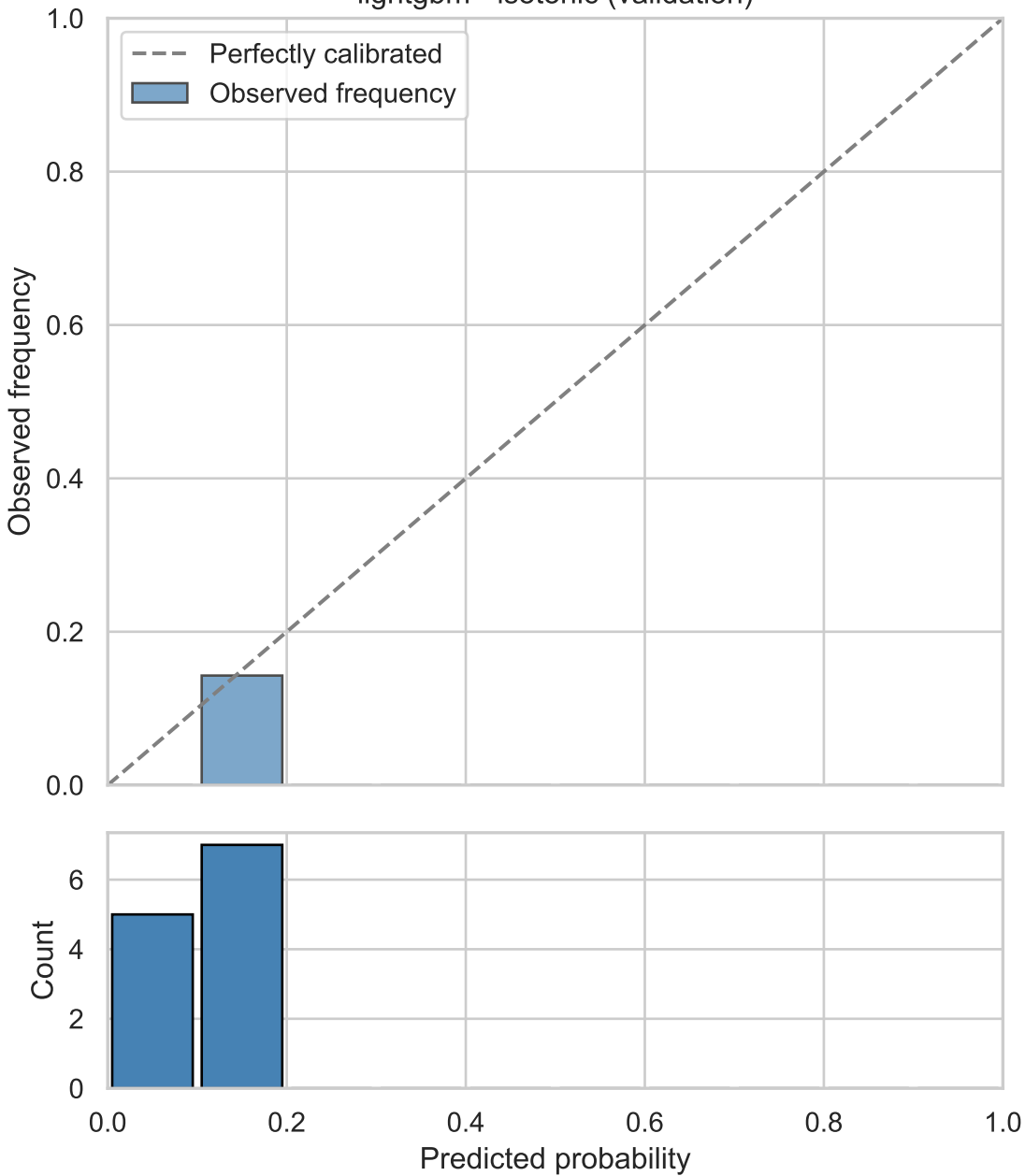
lightgbm - isotonic (validation)
