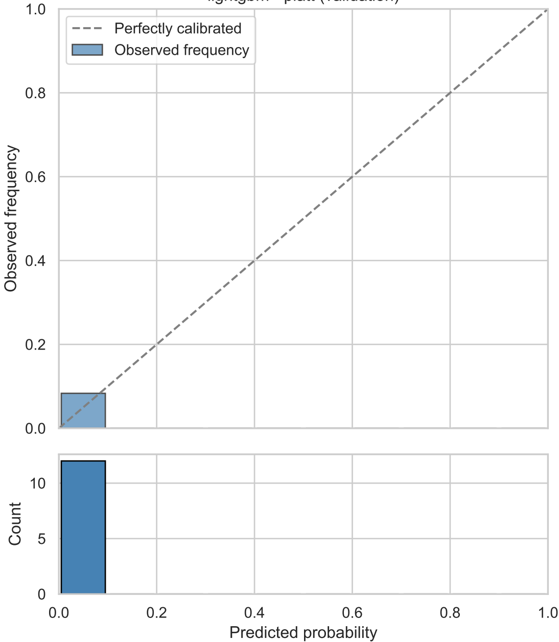
lightgbm - platt (validation)
