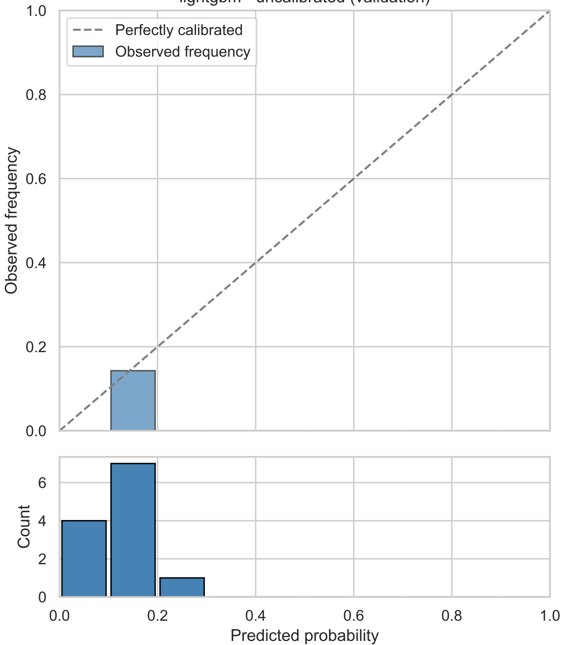
lightgbm - uncalibrated (validation)
