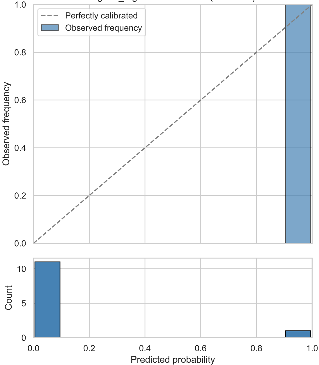
logistic_regression - isotonic (validation)
