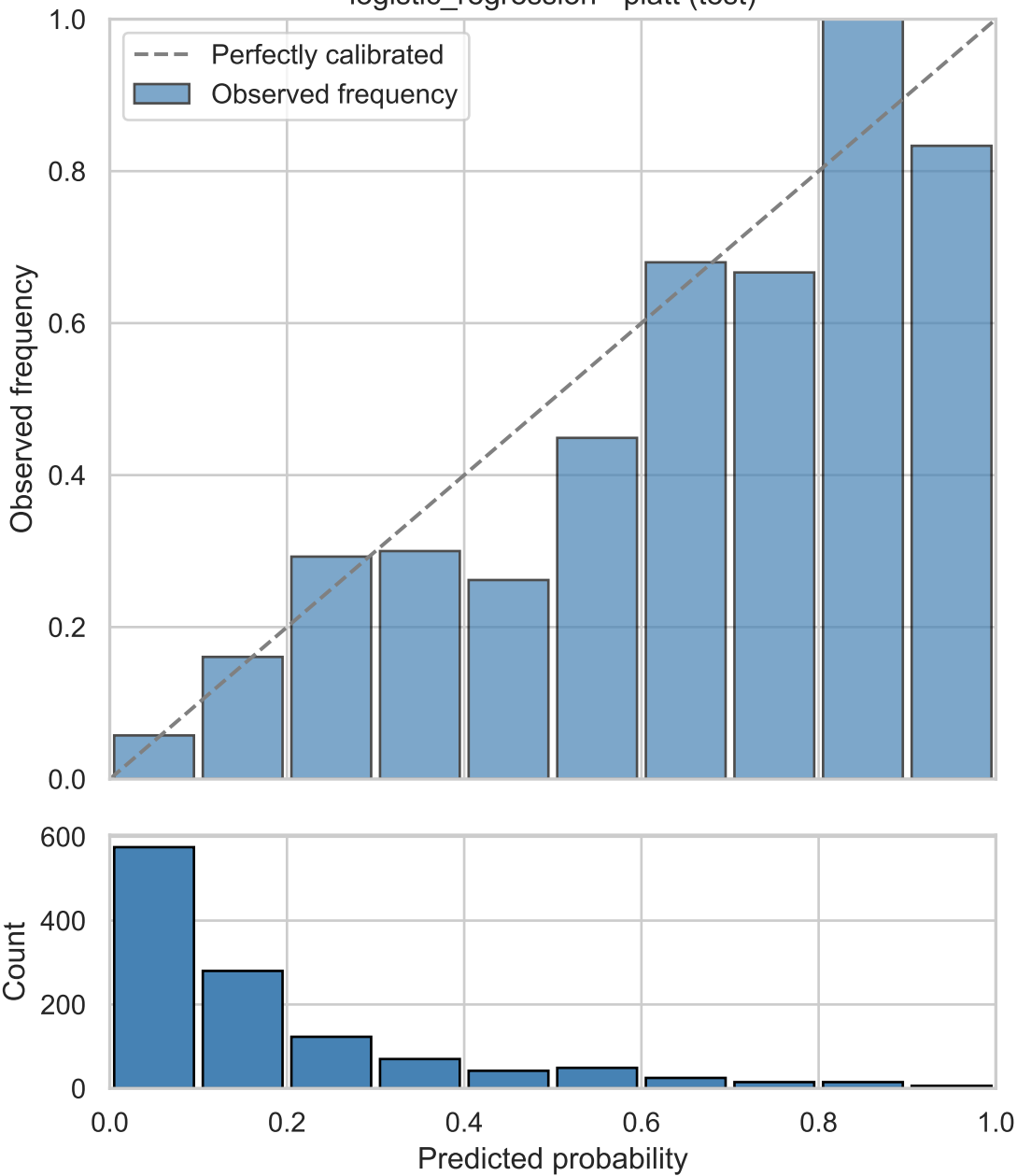
logistic_regression - platt (test)
