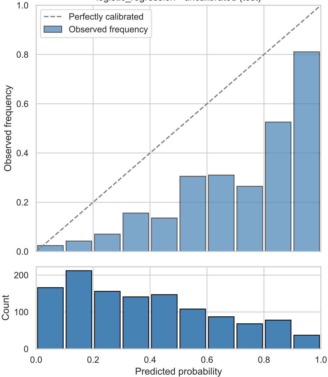
logistic_regression - uncalibrated (test)
