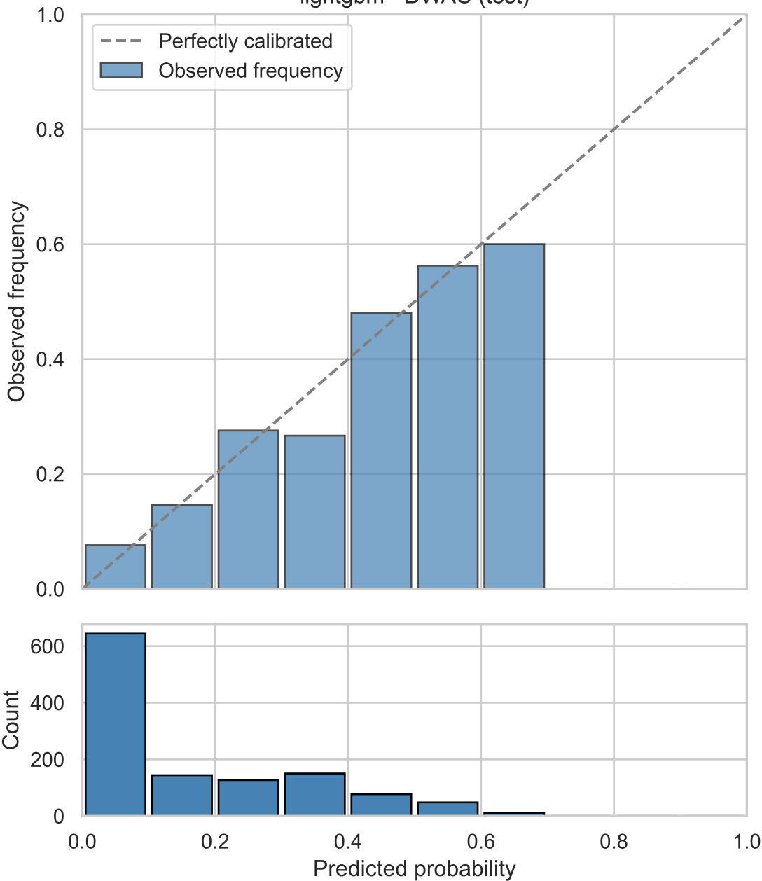
lightgbm - DWAC (test)
