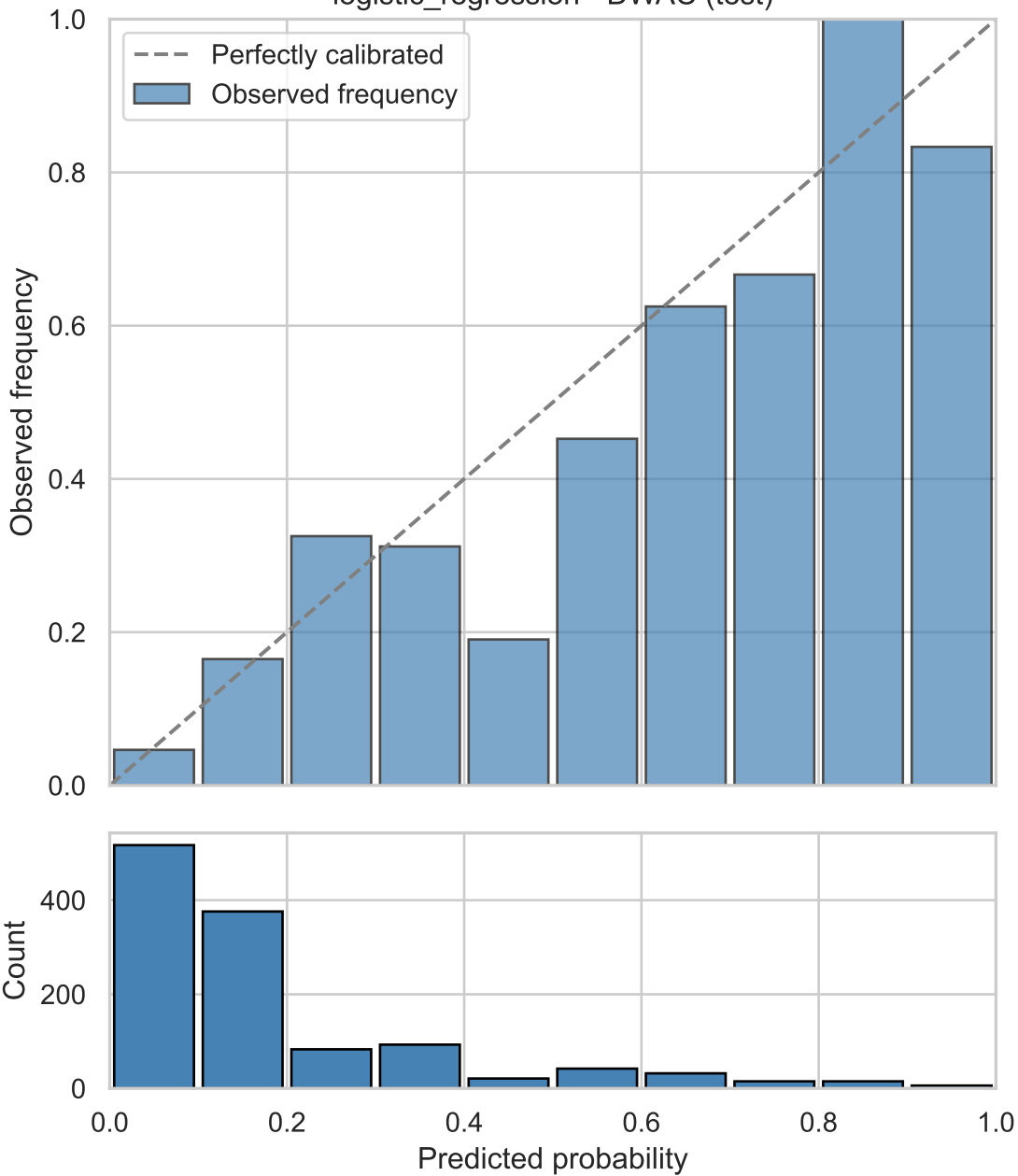
logistic_regression - DWAC (test)
