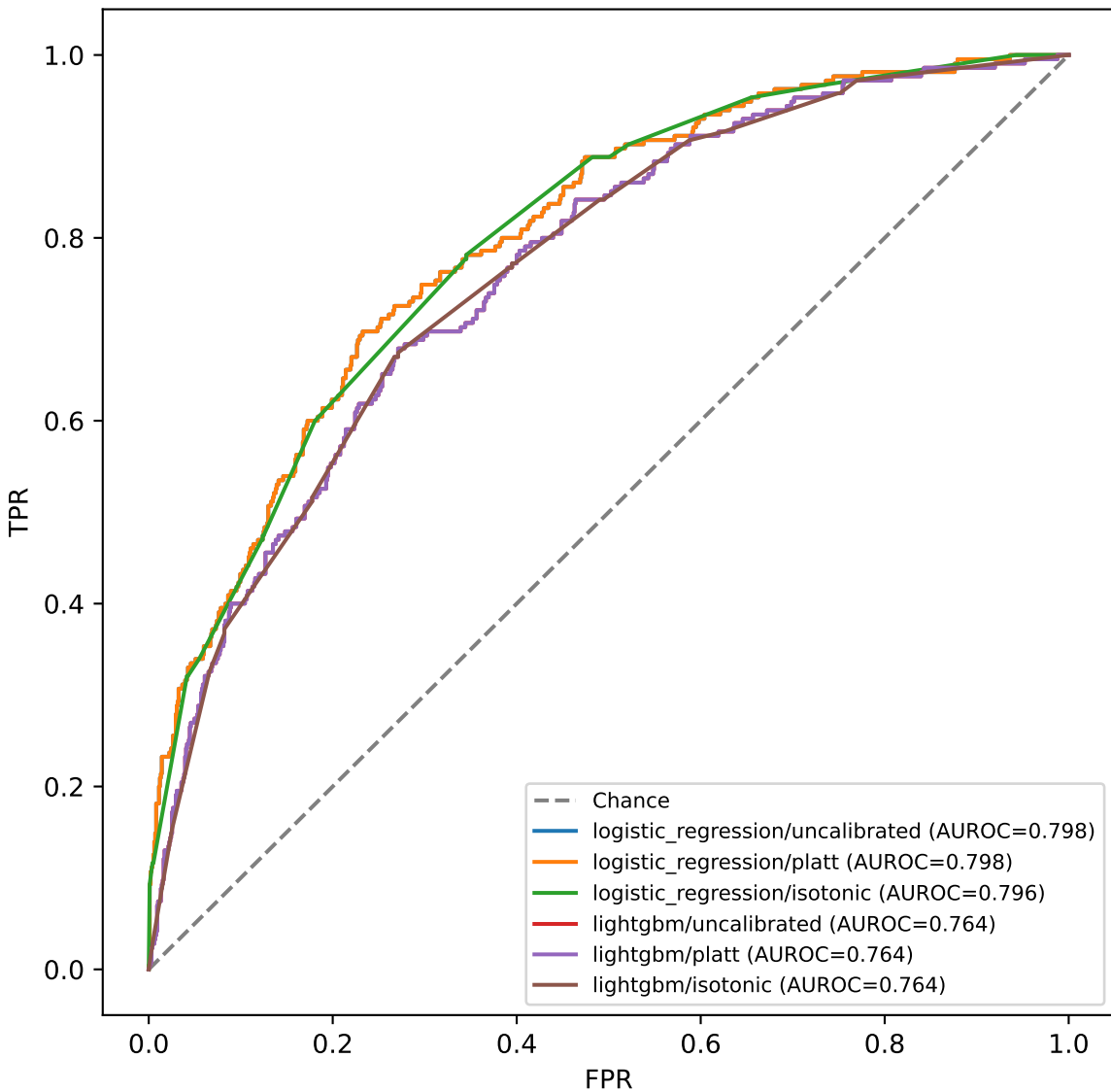
ROC - Test Set
