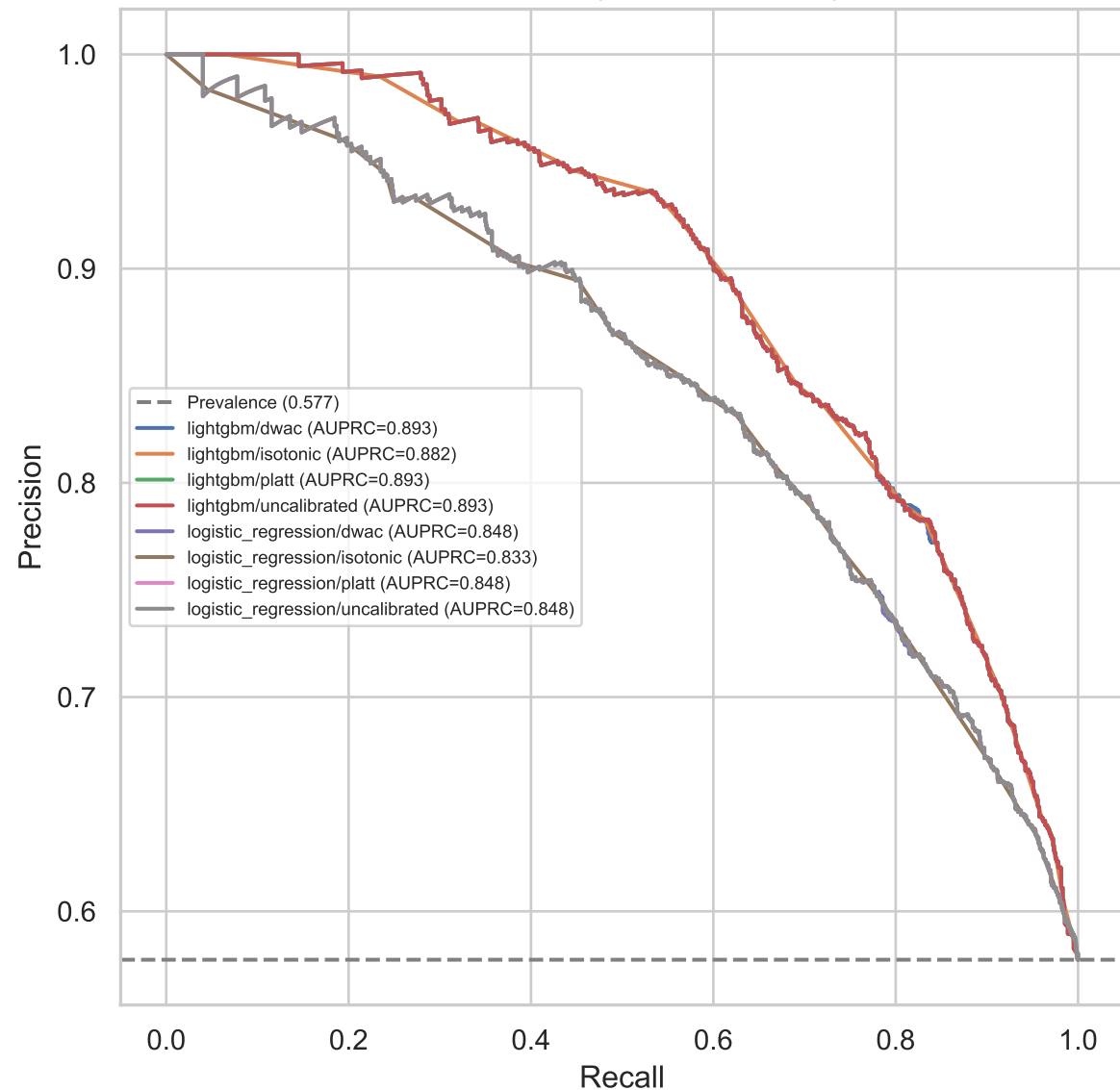
PR - Test Set (full data, n=2158)
