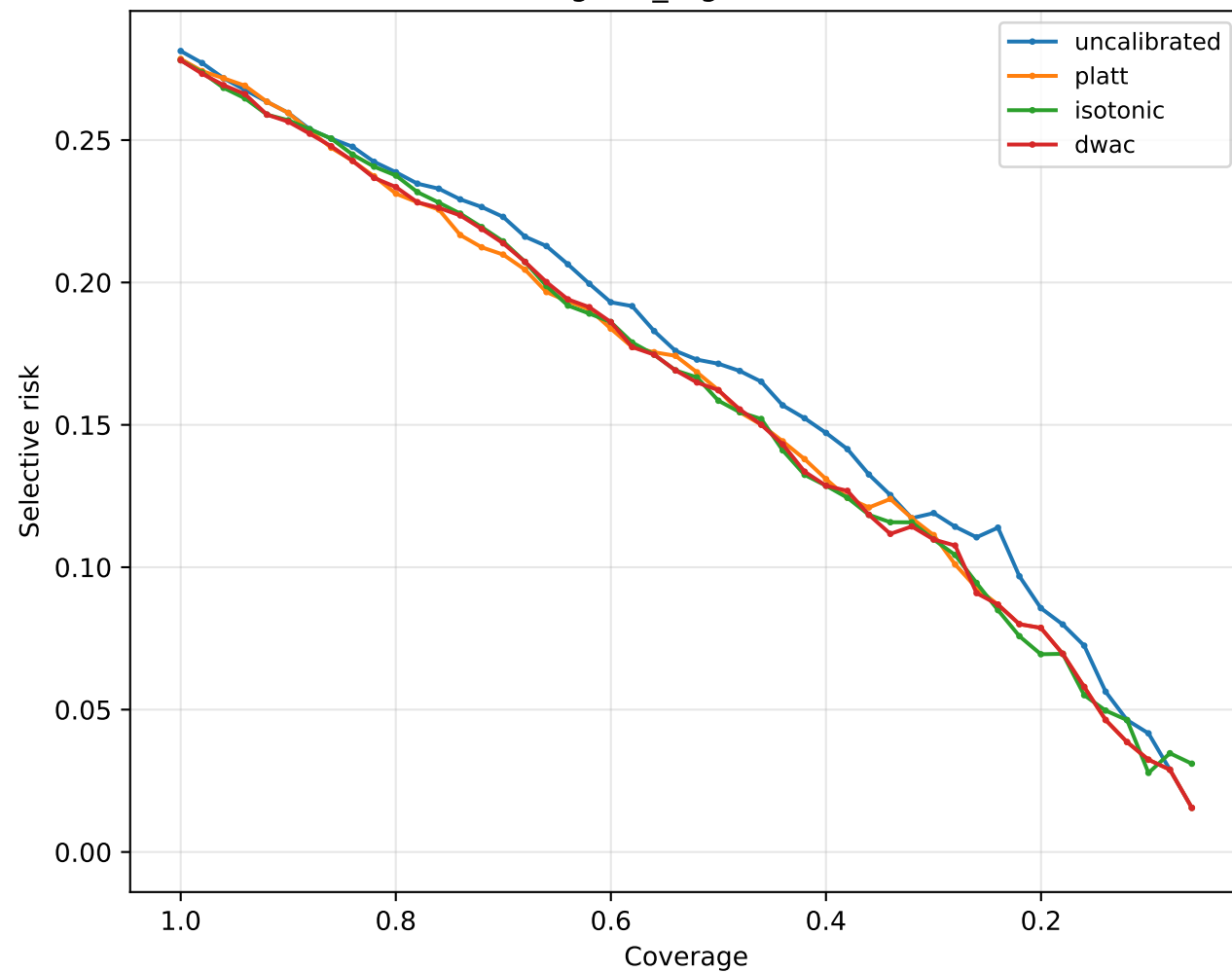
logistic_regression
