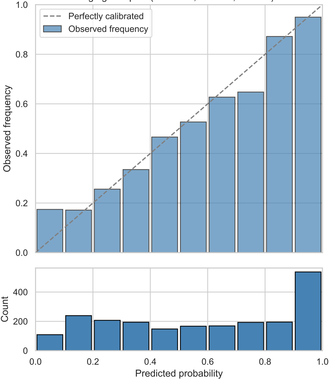
lightgbm - platt (TEST set, full data, n=2158)
