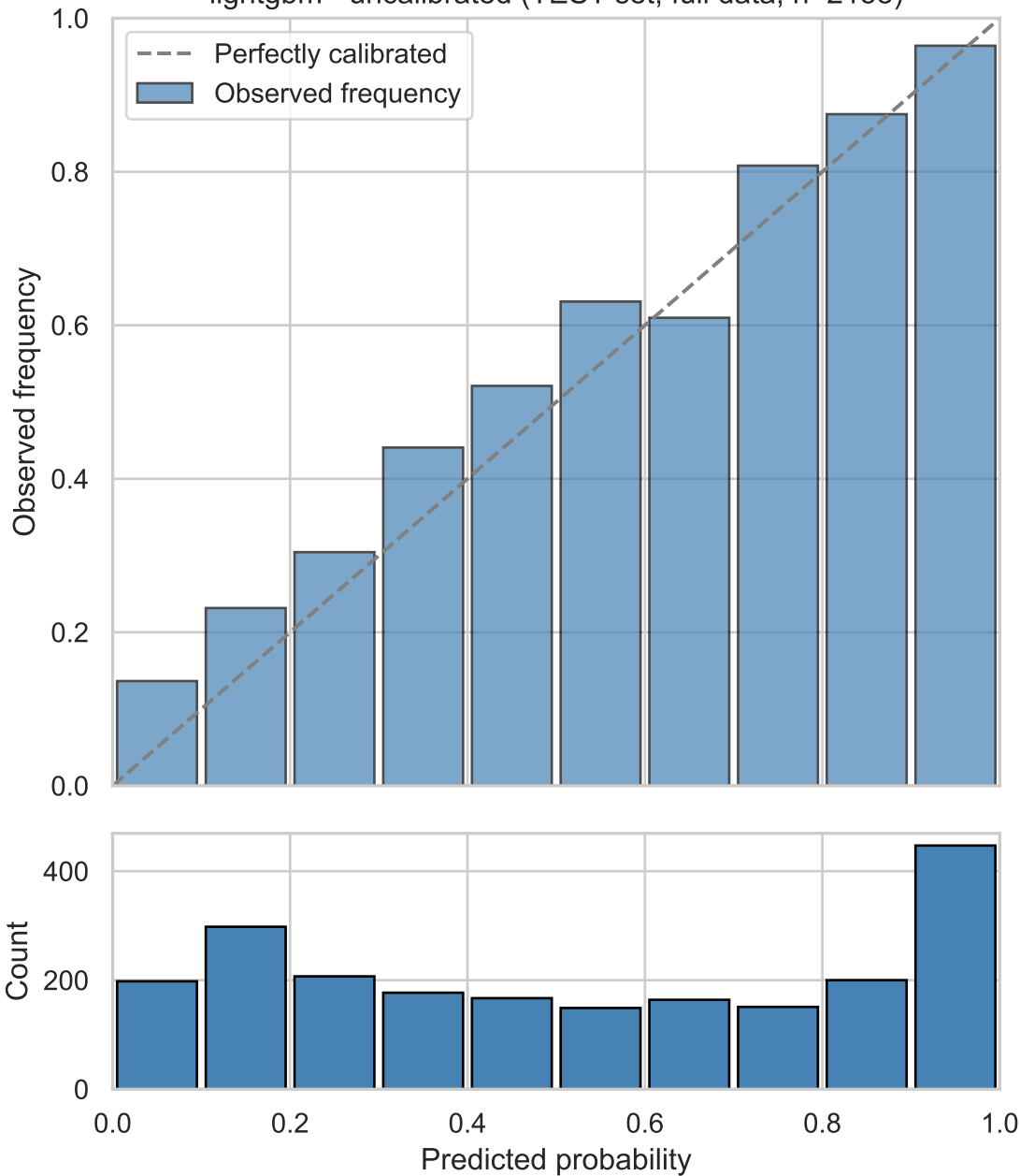
lightgbm - uncalibrated (TEST set, full data, n=2158)
