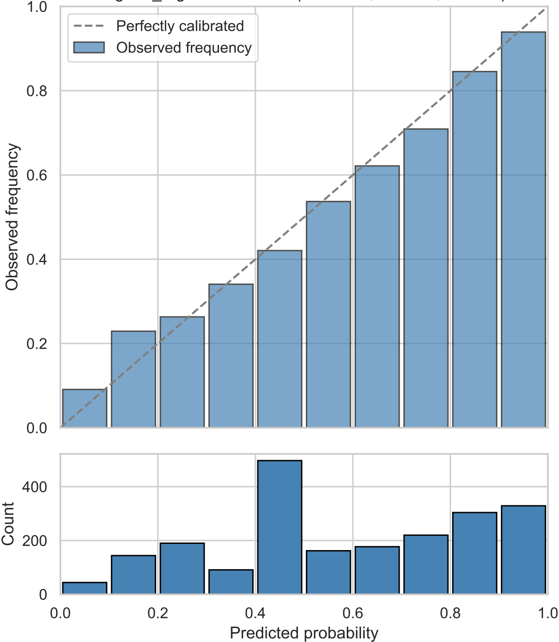
logistic_regression - dwac (TEST set, full data, n=2158)
