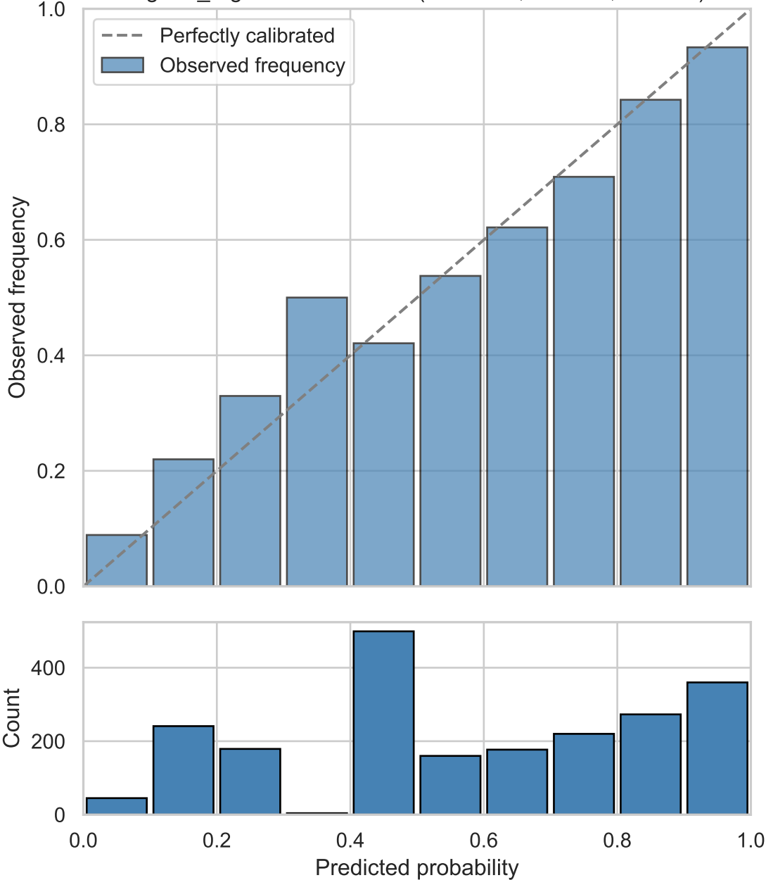
logistic_regression - isotonic (TEST set, full data, n=2158)
