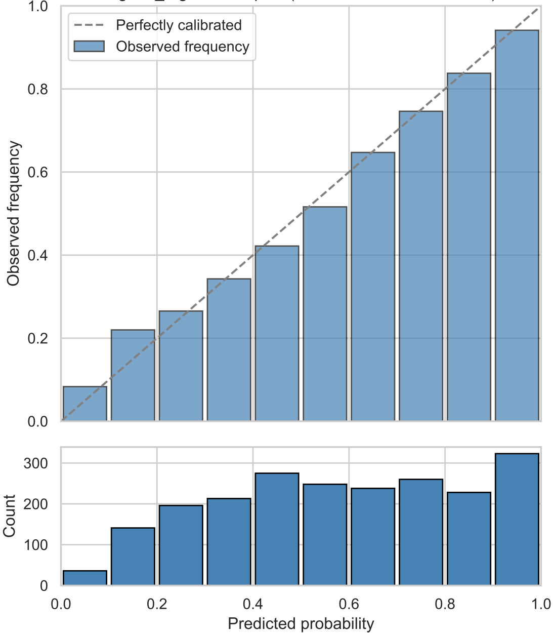
logistic_regression - platt (TEST set, full data, n=2158)
