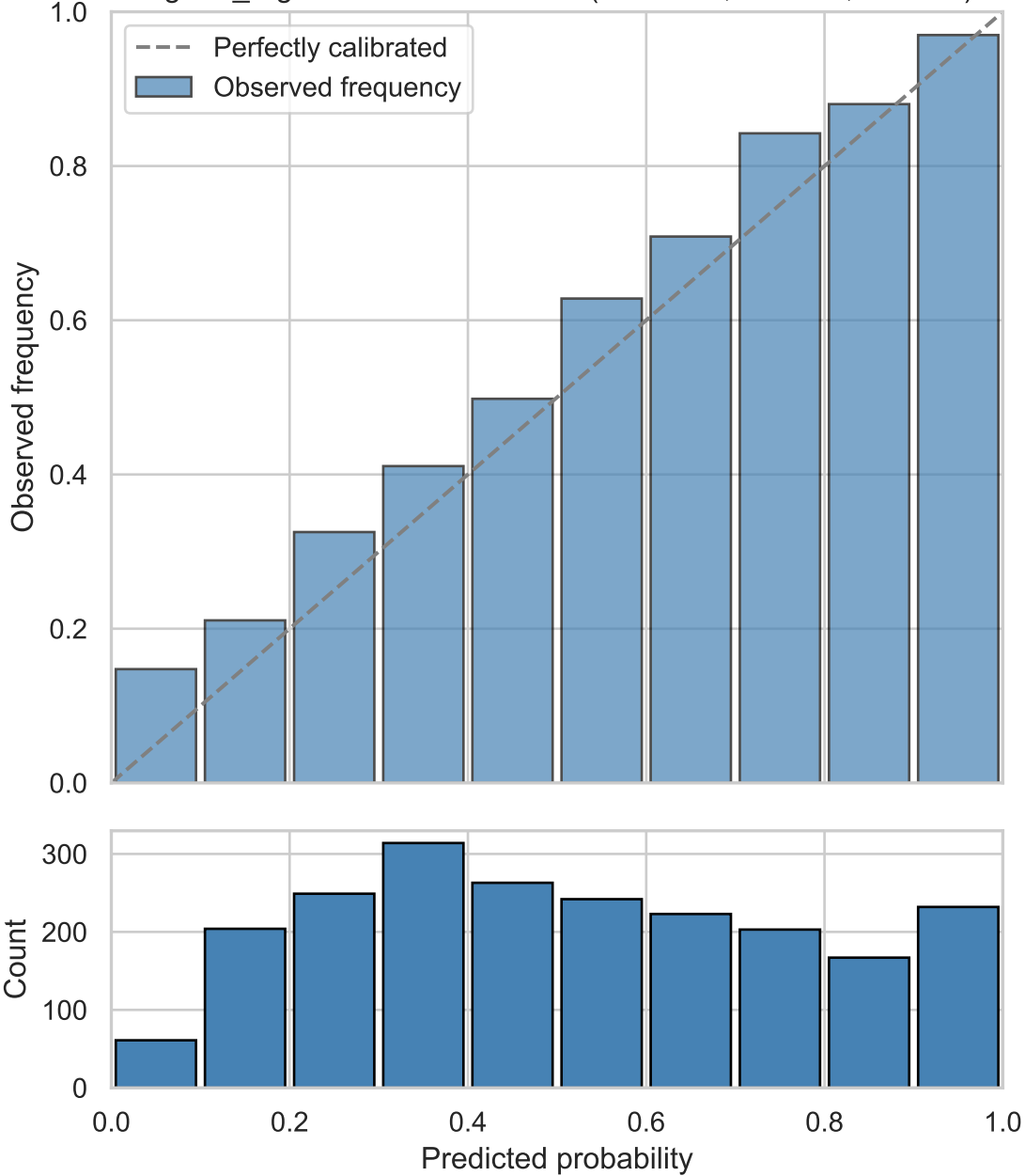
logistic_regression - uncalibrated (TEST set, full data, n=2158)
