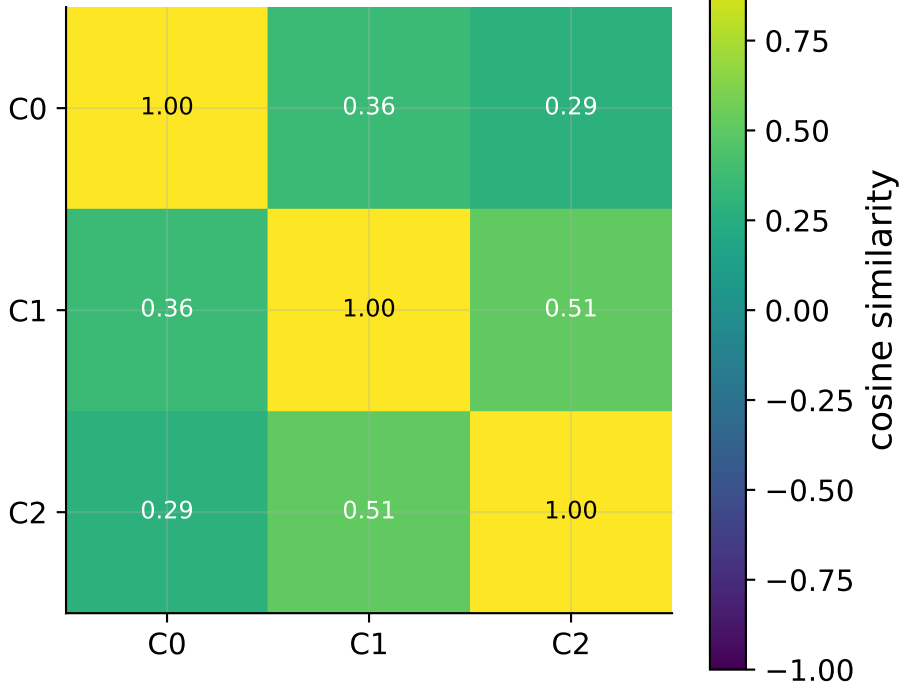
F4: FedSAA client similarity S (mean over 20 layers)
