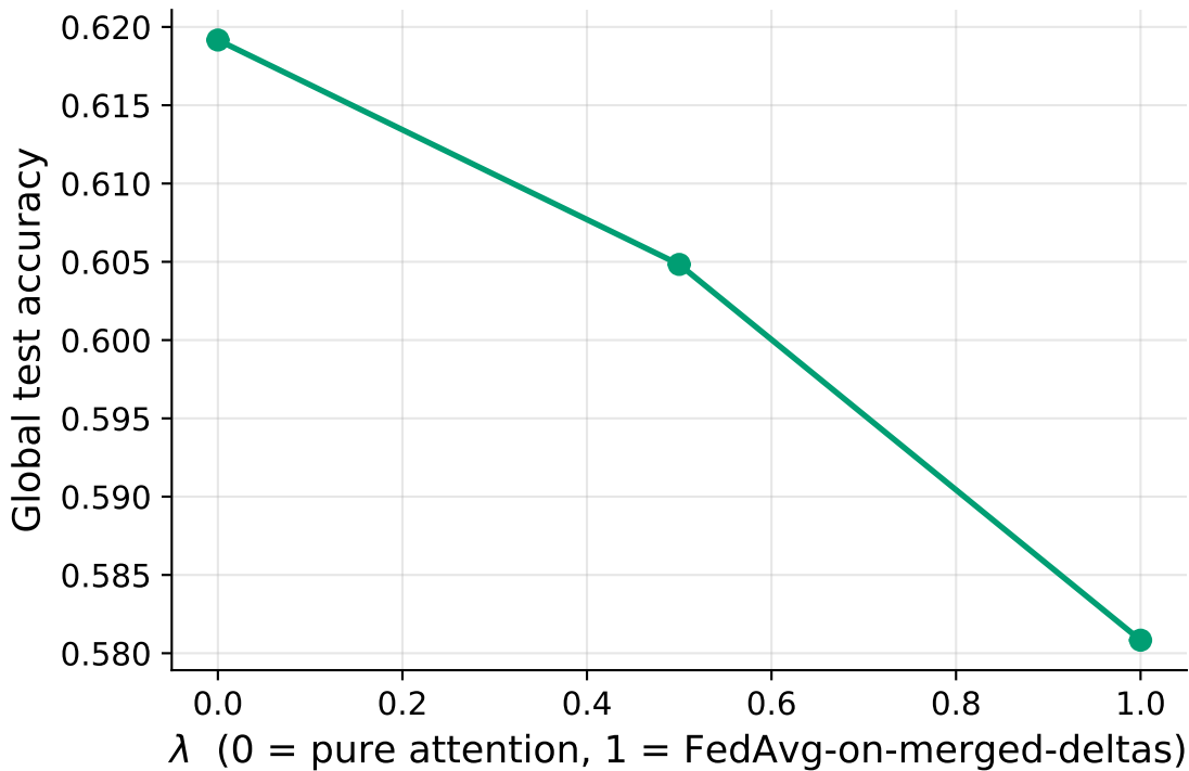
F5: FedSAA lambda ablation (tau=0.1, rank=4, C=1.0)
