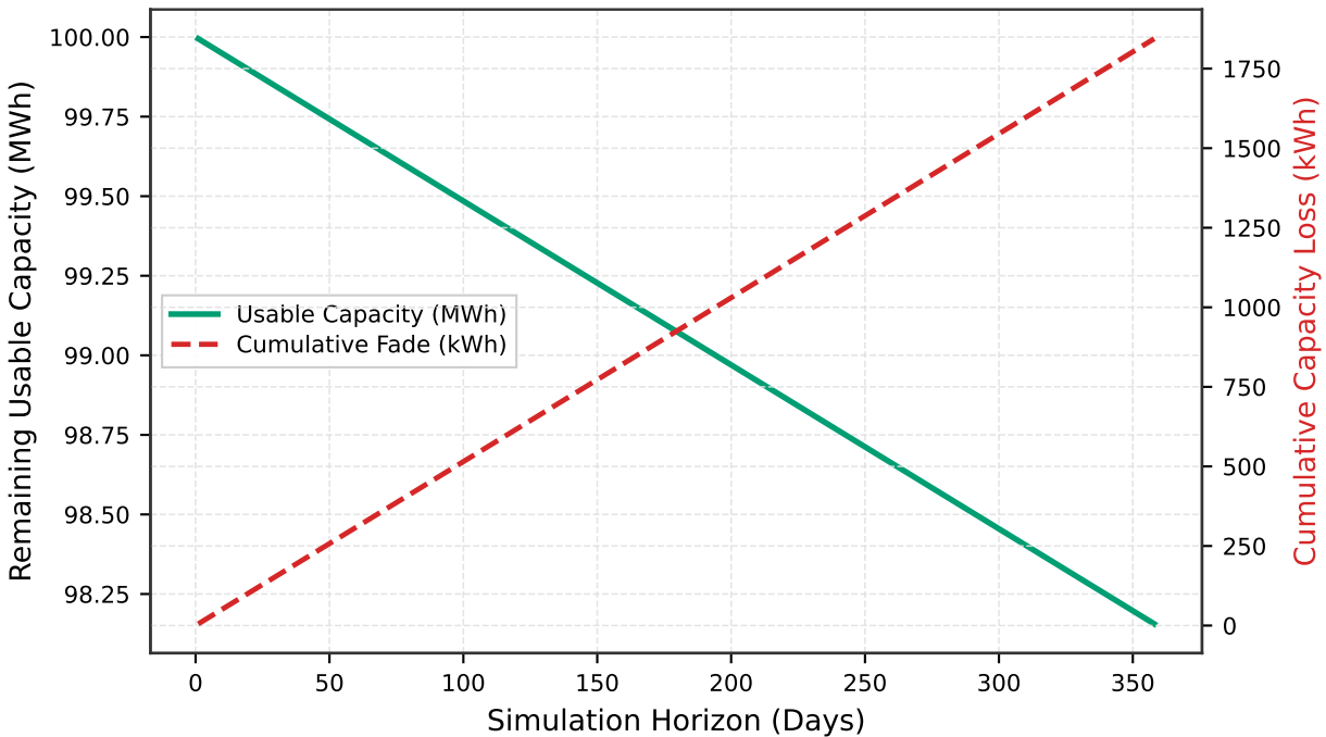
Usable Energy Capacity Attrition & Cumulative Fade
