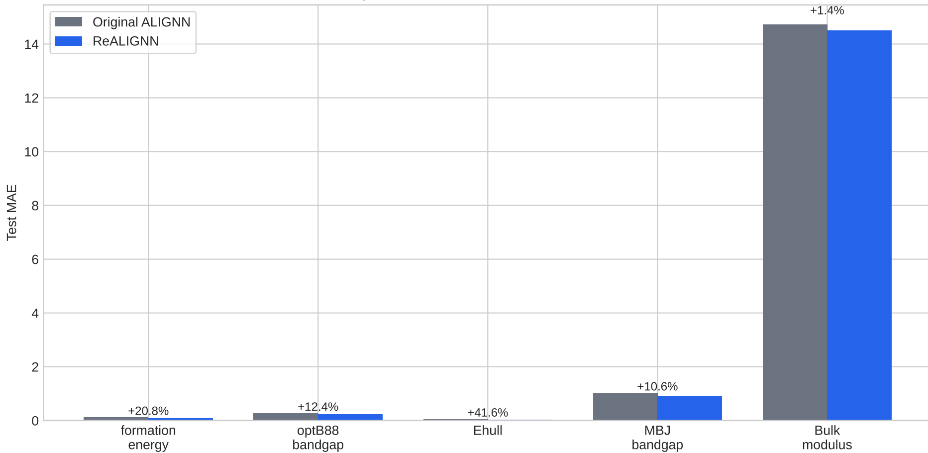
Original ALIGNN vs ReALIGNN: Test MAE
