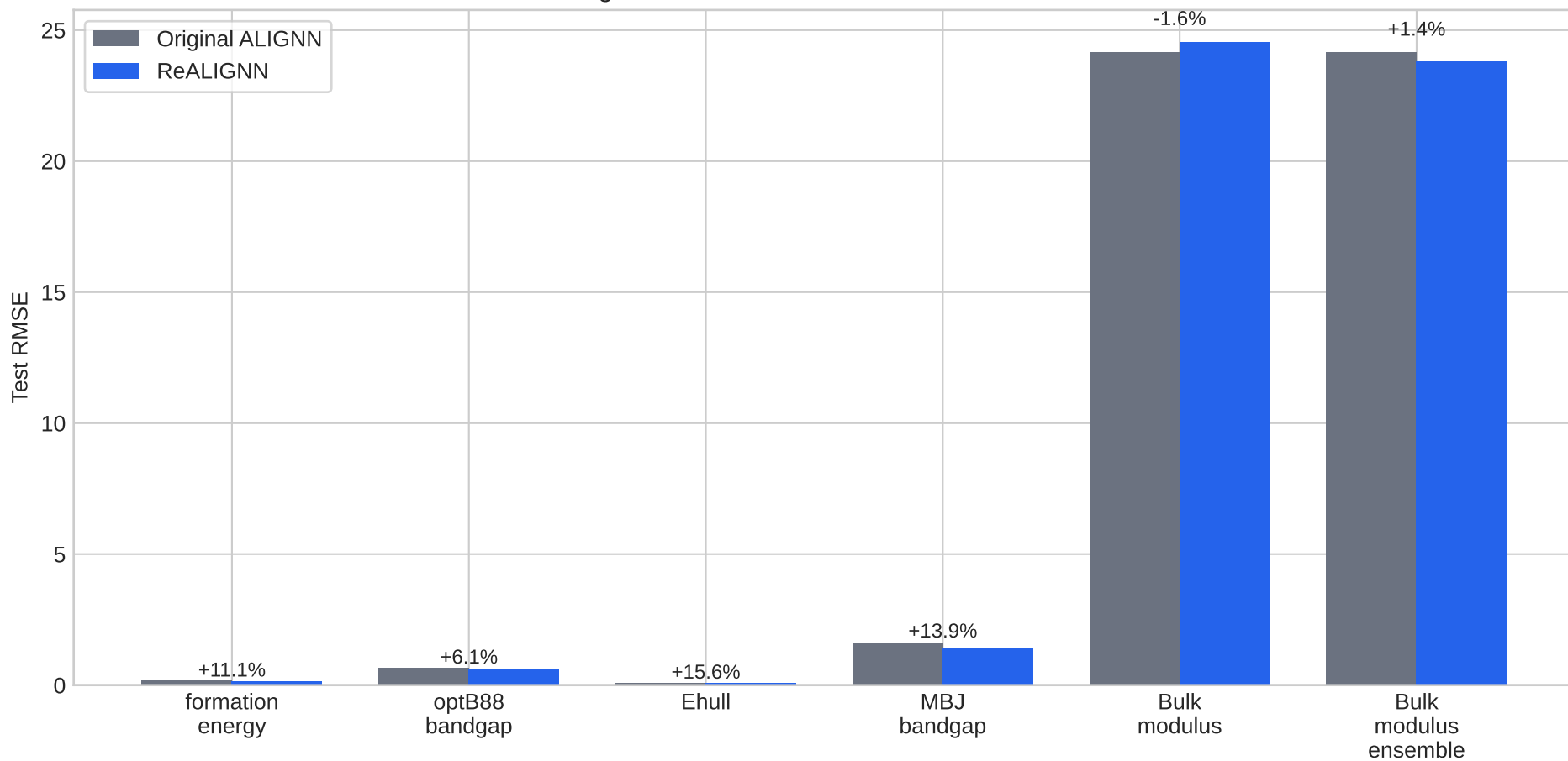
Original ALIGNN vs ReALIGNN: Test RMSE
