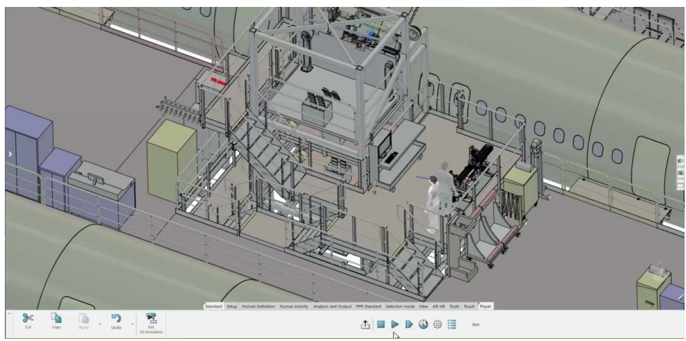
Flextrack robot installation for FAL Mobile
