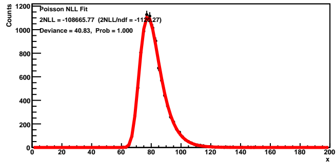
Gumbel Distribution (NLL Fit)
