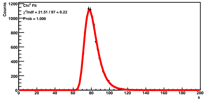
Gumbel Distribution (Chi2 Fit)
