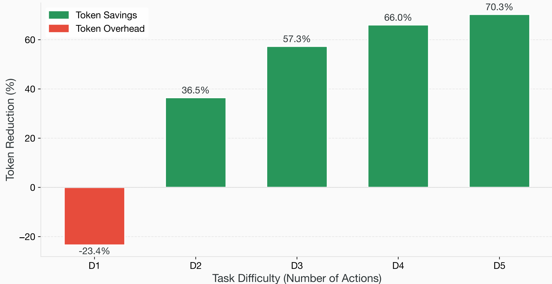
Token Reduction by Difficulty (Multi-Step vs Single-Step)
