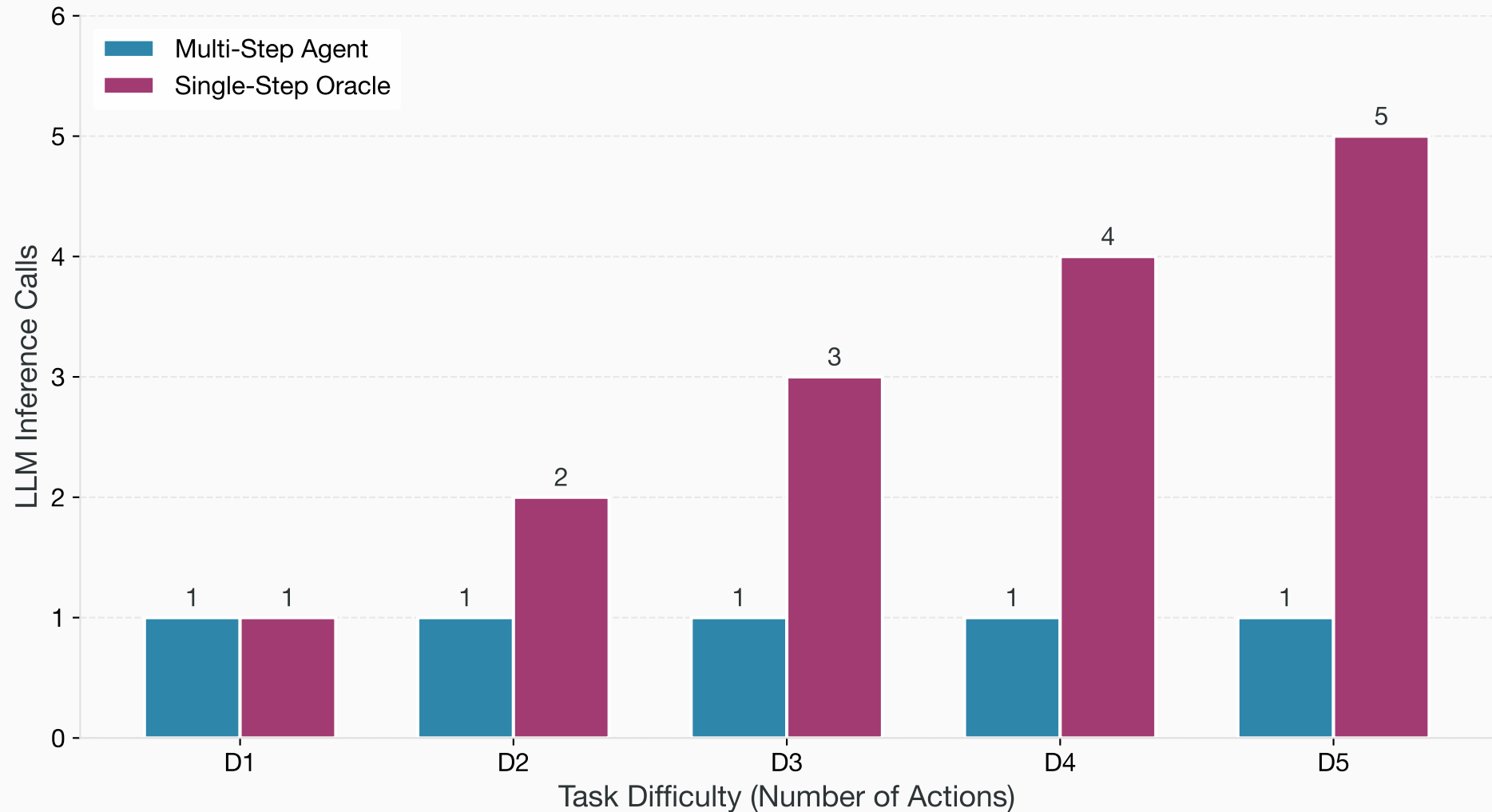
LLM Inference Calls: Multi-Step vs Single-Step Agents
