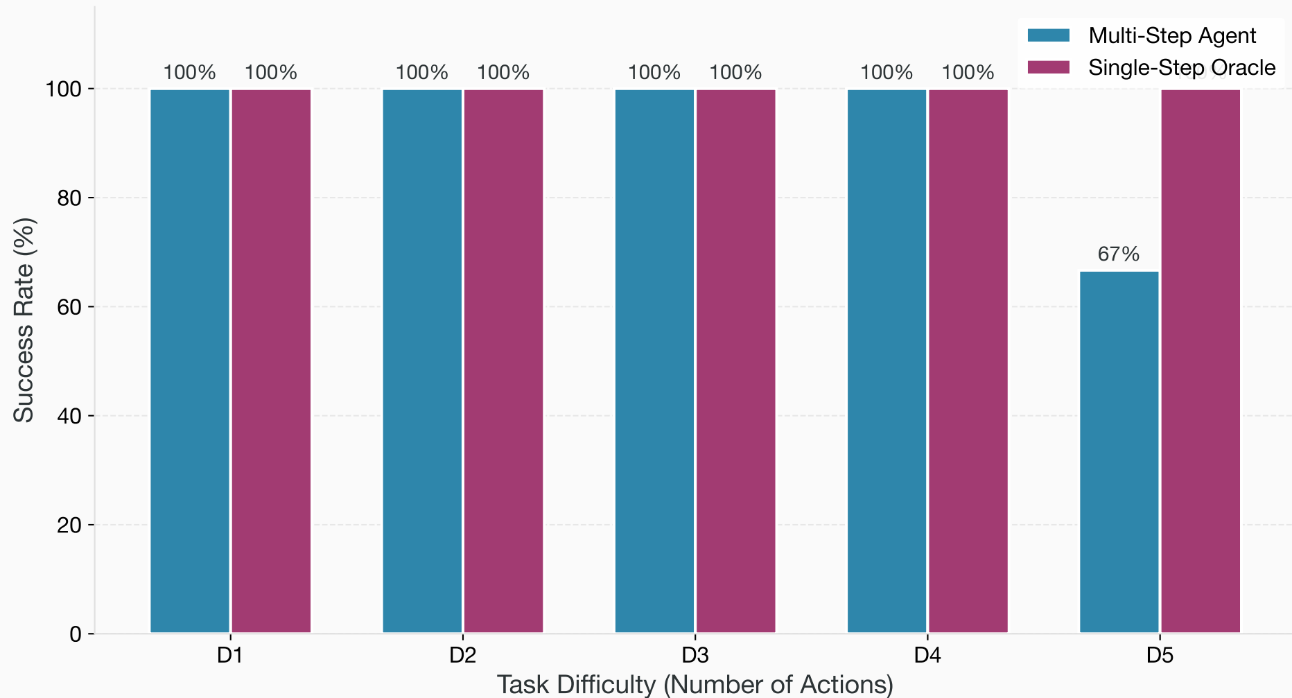
Success Rate Comparison: Multi-Step vs Single-Step Agents
