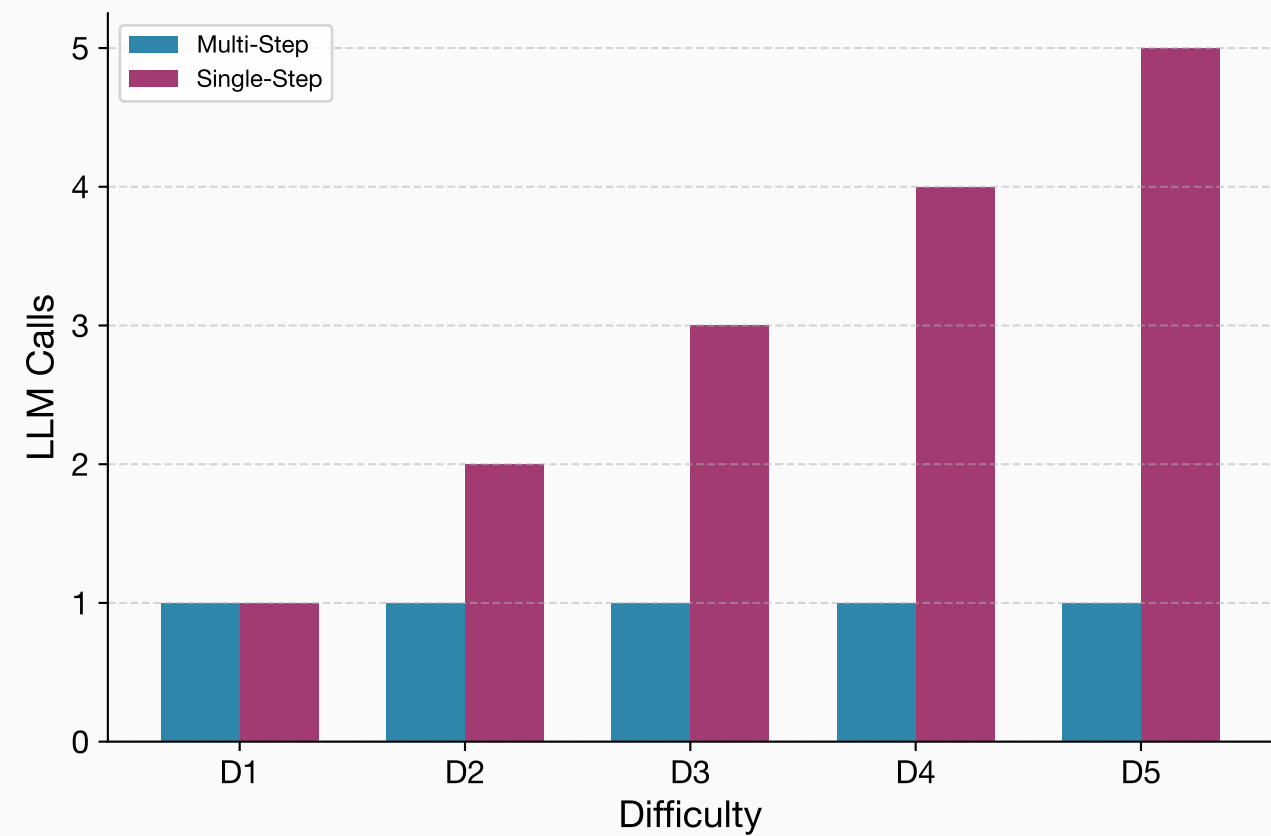
LLM Inference Calls
