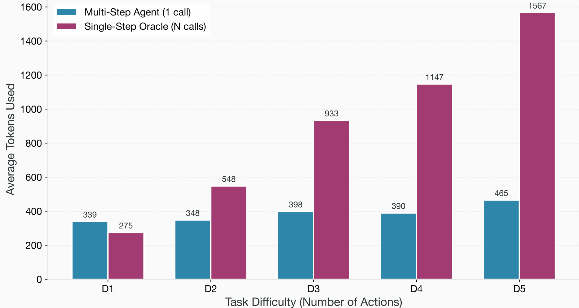
Token Consumption: Multi-Step vs Single-Step Agents
