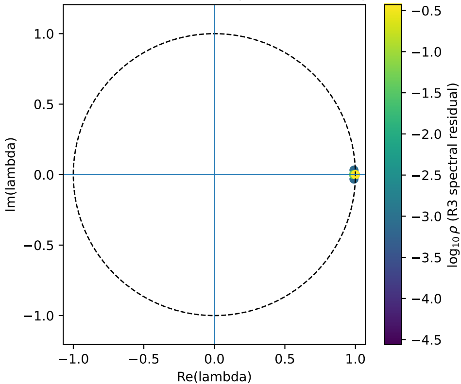
R3 residual-verified KAHKM spectrum: duffing, nlms
